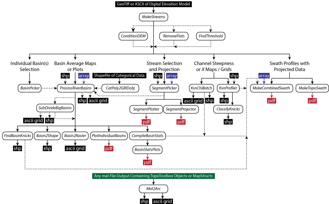
Figure 2: Suggested workflows through TAK functions depending on desired outcome and purpose of analysis. Also highlighted are the nature of the outputs produced by different functions. Definitions of inputs and outputs: shp - a shapefile containing vector data, the geometry of which, e.g. points, lines, polygons, depends on the tool in question; array - a Matlab array, i.e. a matrix of numbers; ascii grid - an ESRI Ascii text file that is interpretable as gridded raster data with projection information by many GIS programs; pdf - a figure output as a PDF.
