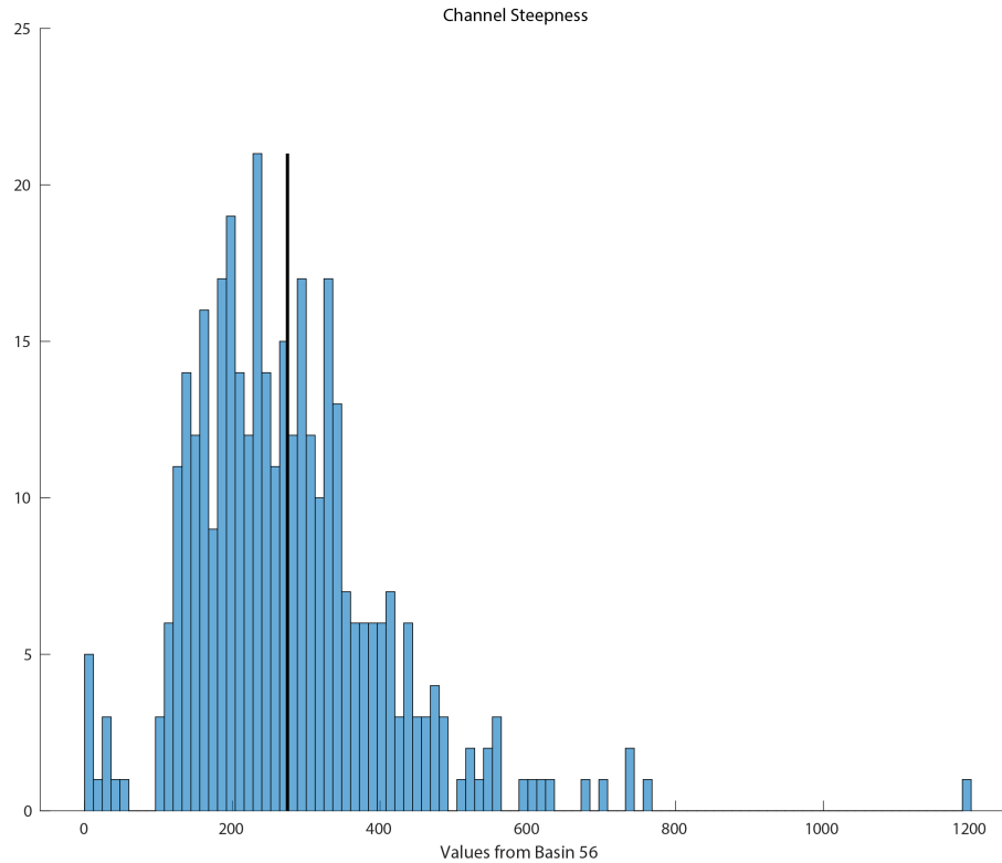
Figure 19: Sample output of 'compare_mean_and_dist' plot from BasinStatsPlots comparing the distribution of k_{sm} within Basin 56 (in the Southern California dataset) to the mean k_{sm} within that basin (the thick black line).
