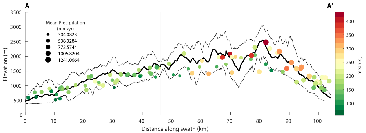
Figure 26: Swath output from MakeCombinedSwath projecting basin locations from CompileBasinStats and colored by mean k_{sn} and scaled by mean precipitation.
