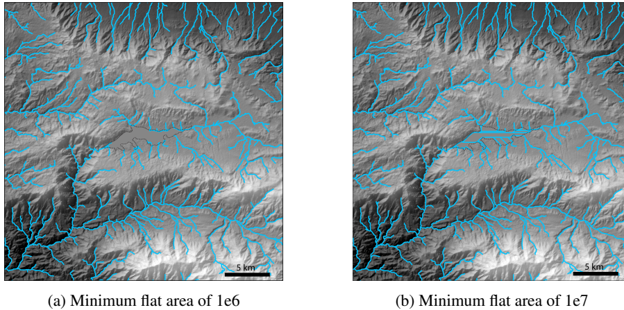
Figure 5: Difference in output of MakeStreams depending on value used for min_flat_area when auto removing flat areas in the area around Big Bear lake (outline of lake is shown in thin dotted black line) in the San Bernadino Mountains. When min_flat_area is 1e6 (5a), the lake is identified as a flat and removed, but when min_flat_area is 1e7 (5b) the lake is not identified as a flat and thus streams are routed through the lake.
