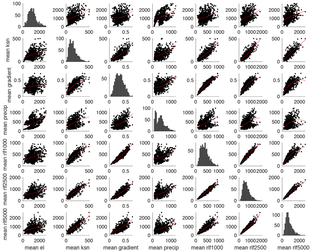
Figure 20: Sample output of 'scatterplot_matrix' plot from BasinStatsPlots . Data is from the Southern California sample dataset using the basins > 100 \text{ km}^2 filtered by trunk confluences > 5 \text{ km}^2 .
