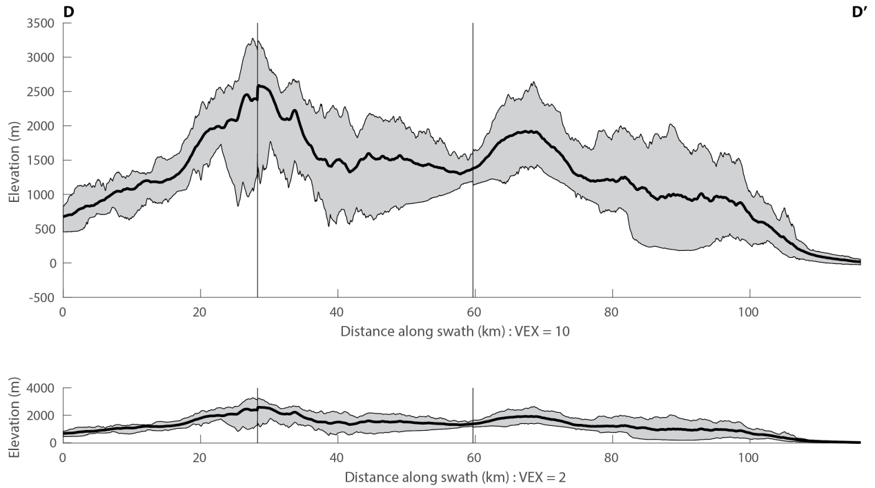
Figure 22: Basic swaths output from MakeTopoSwath highlighting the function of the 'vex' parameter to control the vertical exaggeration.
