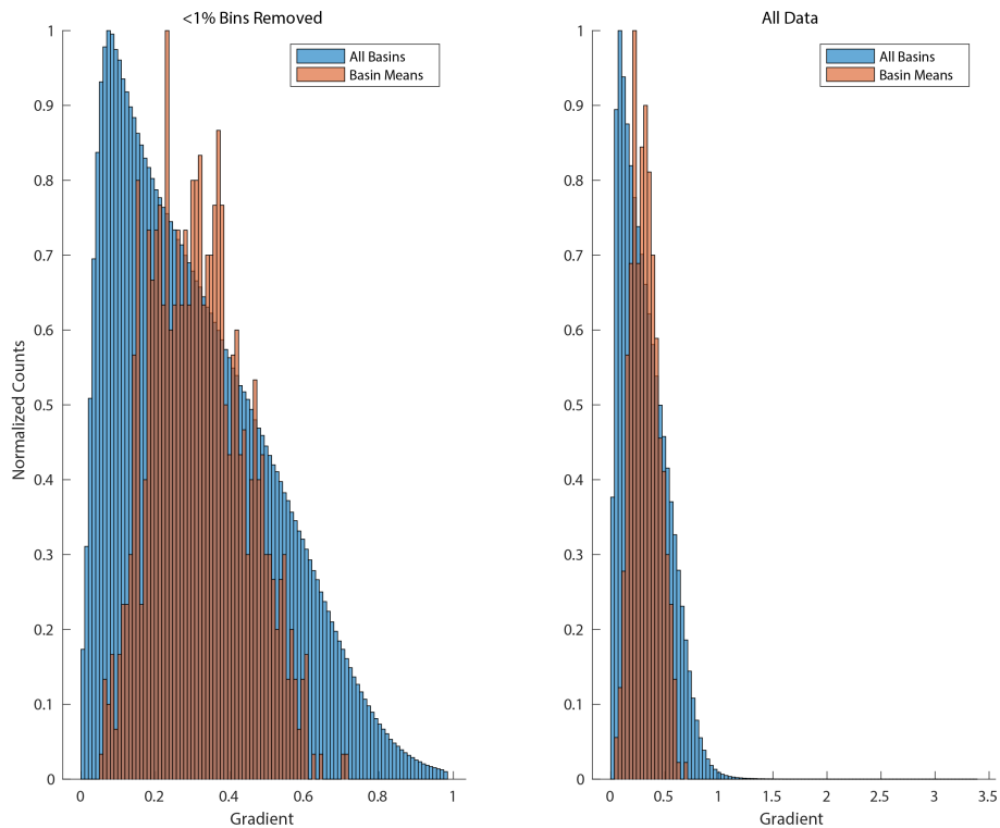
Figure 18: Sample output of ' compare_mean_and_dist ' plot from BasinStatsPlots comparing the distribution of gradient across all nodes in all basins (blue) to the distribution of mean gradients across all basins (orange). Data is from the Southern California sample dataset using the basins > 100 km 2 filtered by trunk confluences > 5 km 2 .
