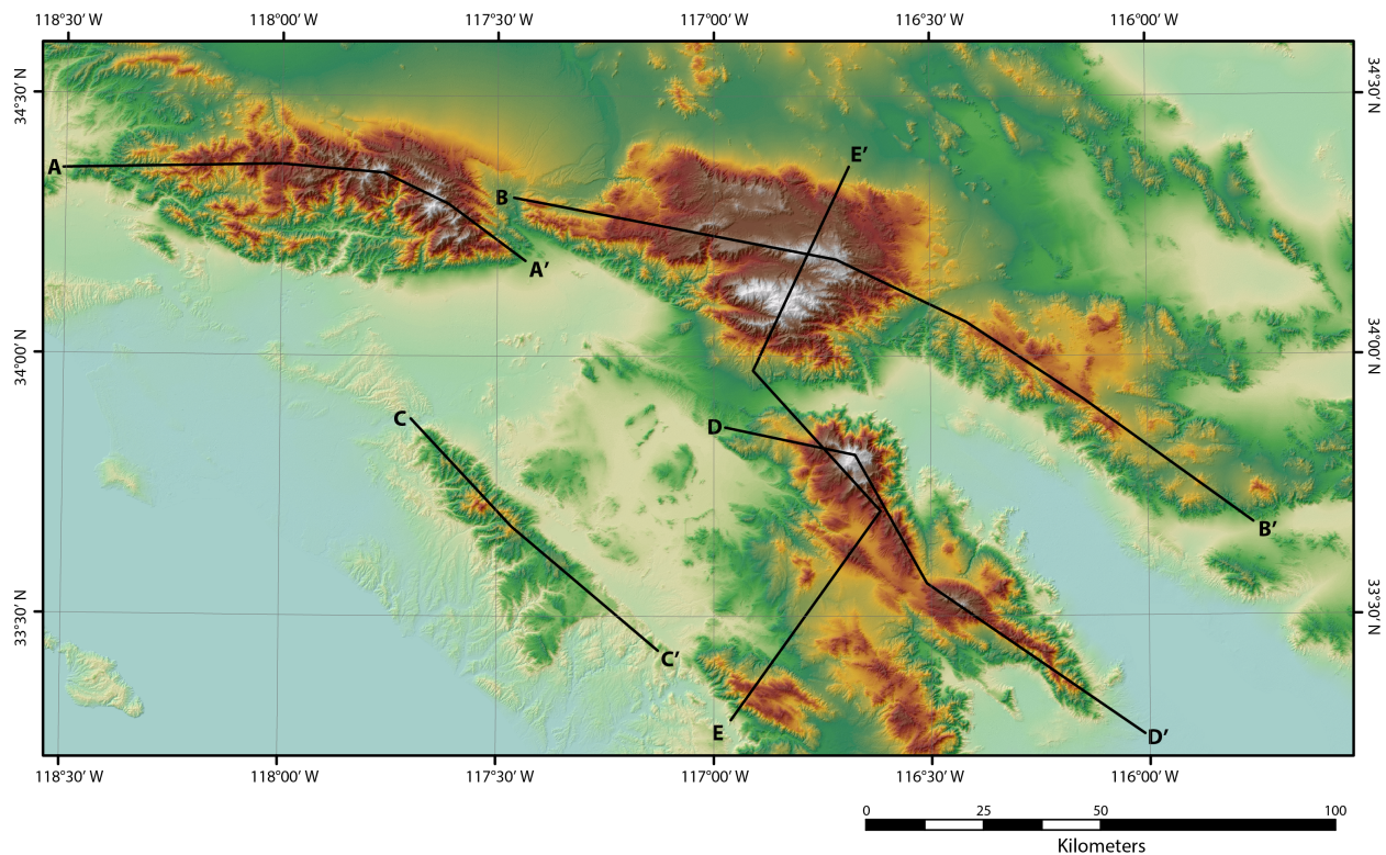
Figure 21: Location of swaths used to demonstrate uses of MakeTopoSwath and MakeCombinedSwath .
