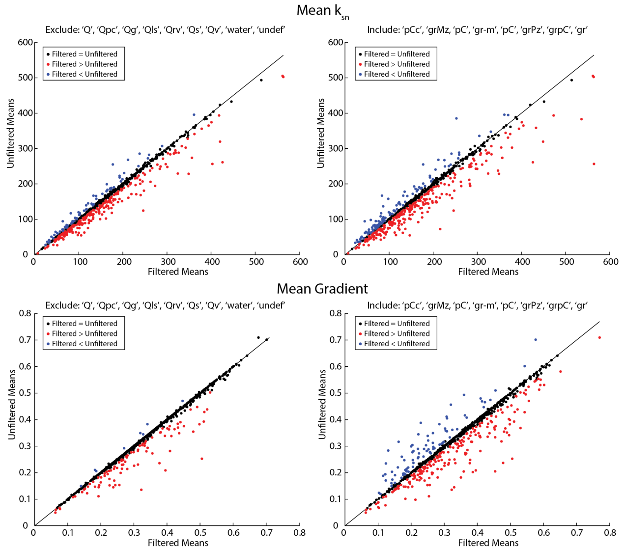
Figure 16: Selected outputs of 'compare_filtered' plot from BasinStatsPlots comparing results of an excluding quaternary, water, and undefined areas vs including basement rocks. Data is from the Southern California sample dataset using the basins > 100 km 2 filtered by trunk confluences > 5 km 2 .
