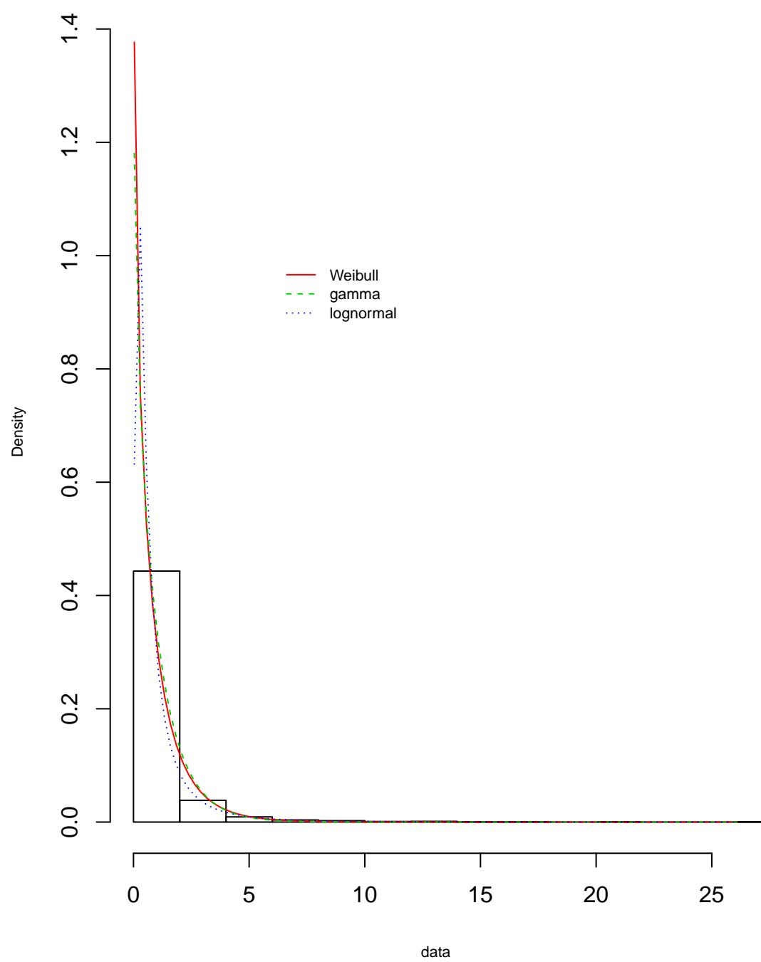
Histogram and theoretical densities
