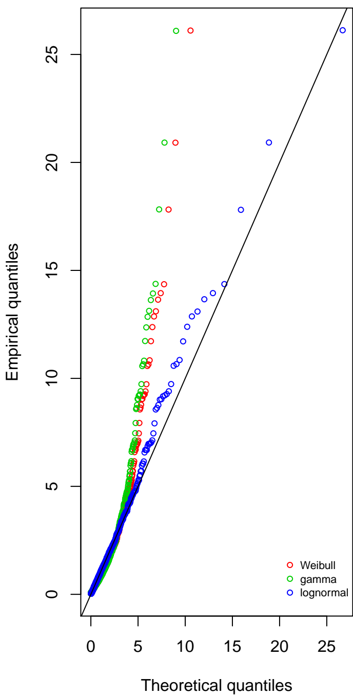
Q-Q plot
