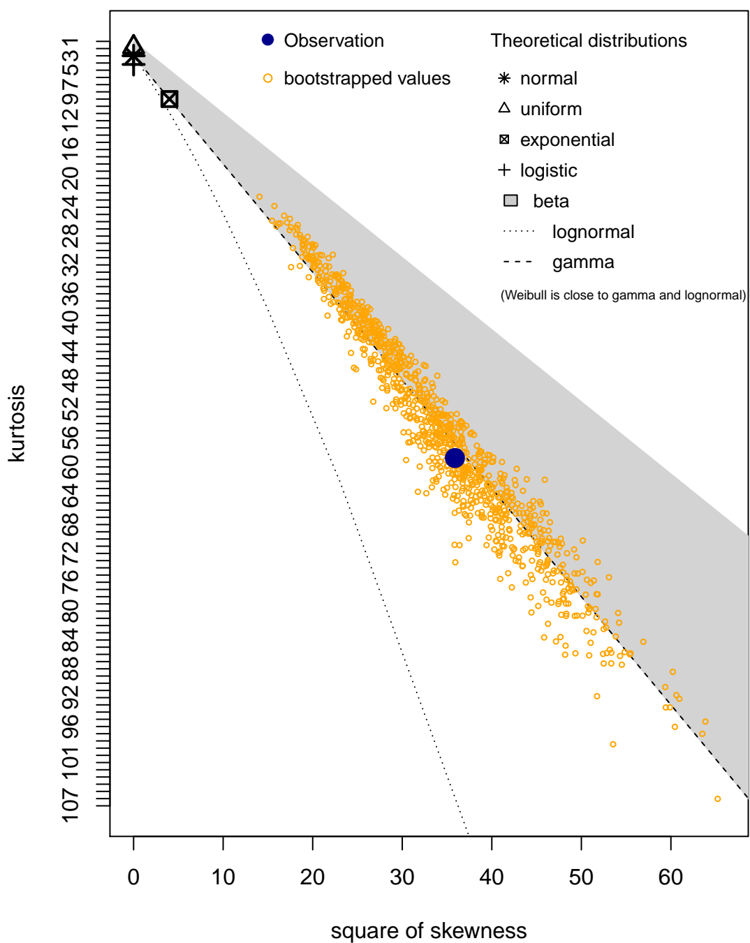
Cullen and Frey graph
