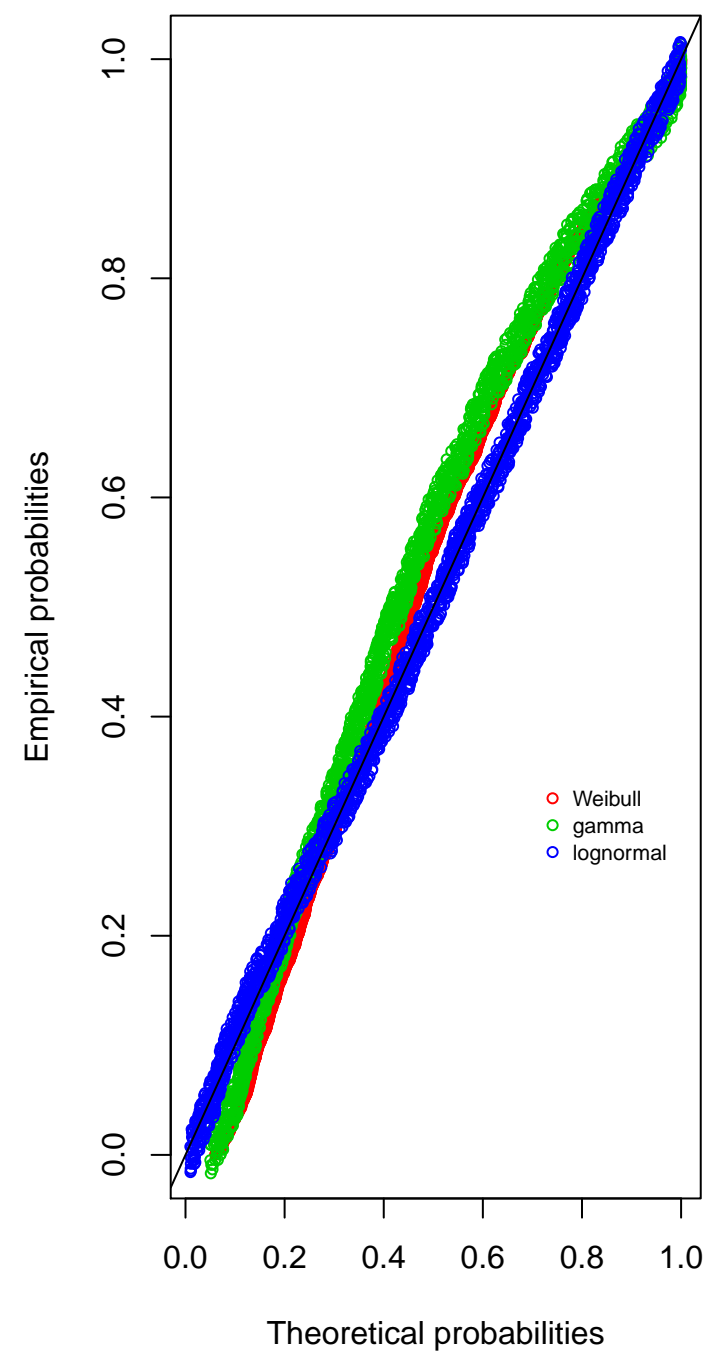
P-P plot
