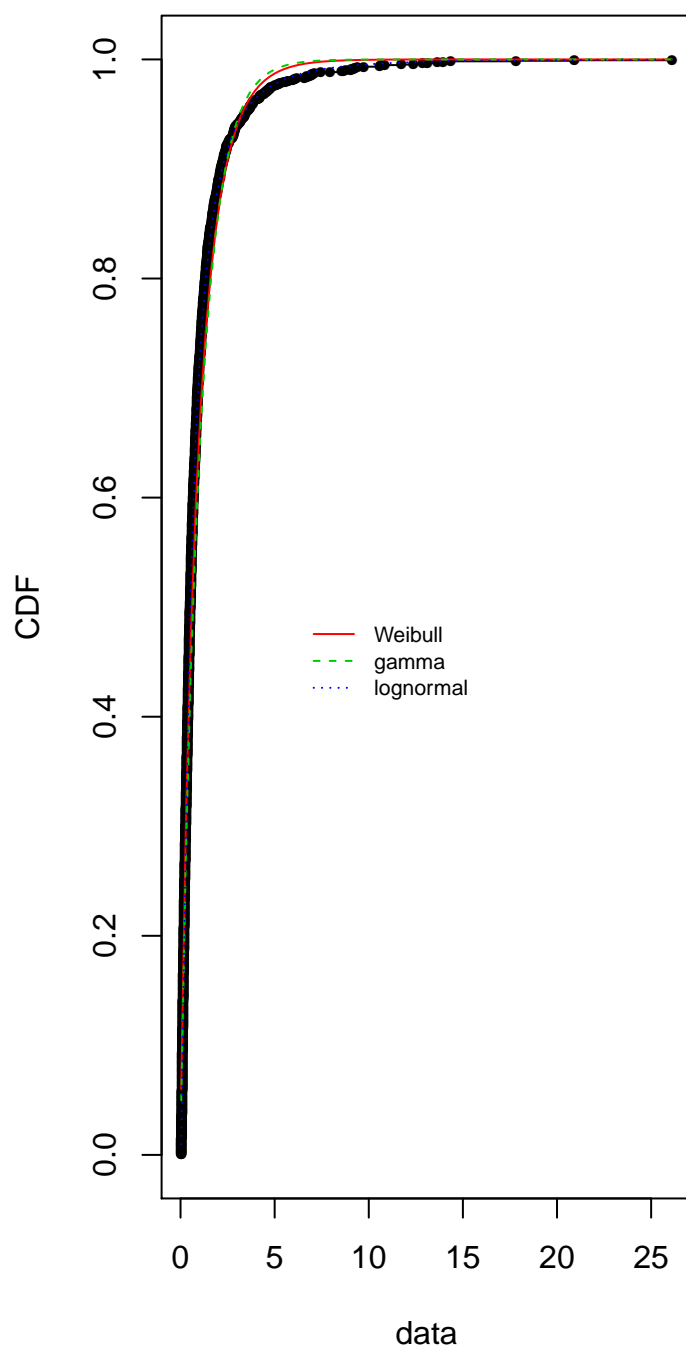
Empirical and theoretical CDFs
