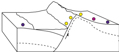
(a) Normal Fault (Ehlers et al., 2003)
