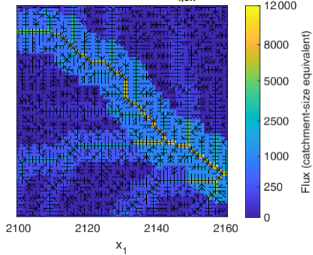
(c) Effective ice flux A_{i,eff}
