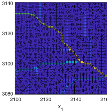
(a) Discharge A_i
