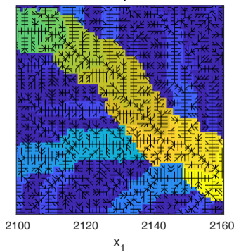
(b) Ice flux A_i (extended)
