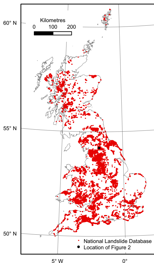
Fig. 1. UK Map showing the distribution of landslide points in the National Landslide Database (NLD) which have undergone quality assurance control at the British Geological Survey. Black
