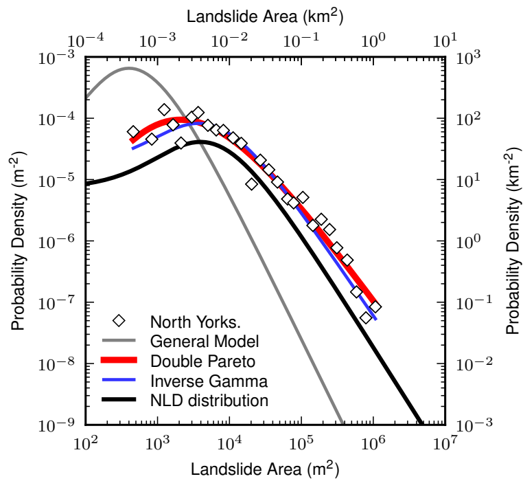
Fig. 5. Probability distribution of landslide deposit area for landslides in North Yorkshire - organized into logarithmically spaced bins (open diamonds). Solid black and grey lines show maximum likelihood esti
