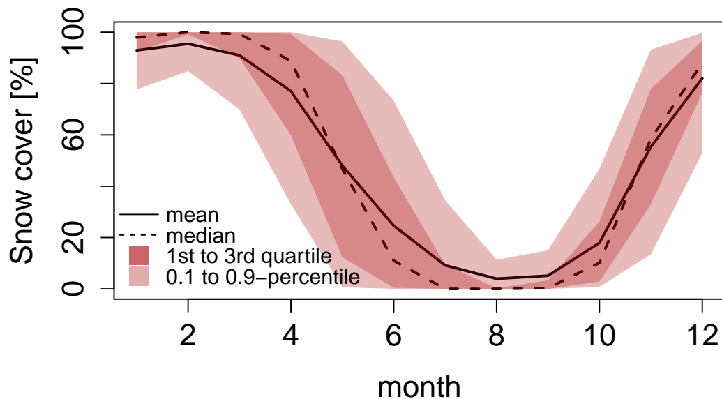
Fig. 1. Gunt catchment snow cover dynamics based on 12 years of MODIS MOD10CM monthly snow cover data. Mean, median and quantiles are given to highlight variability.
