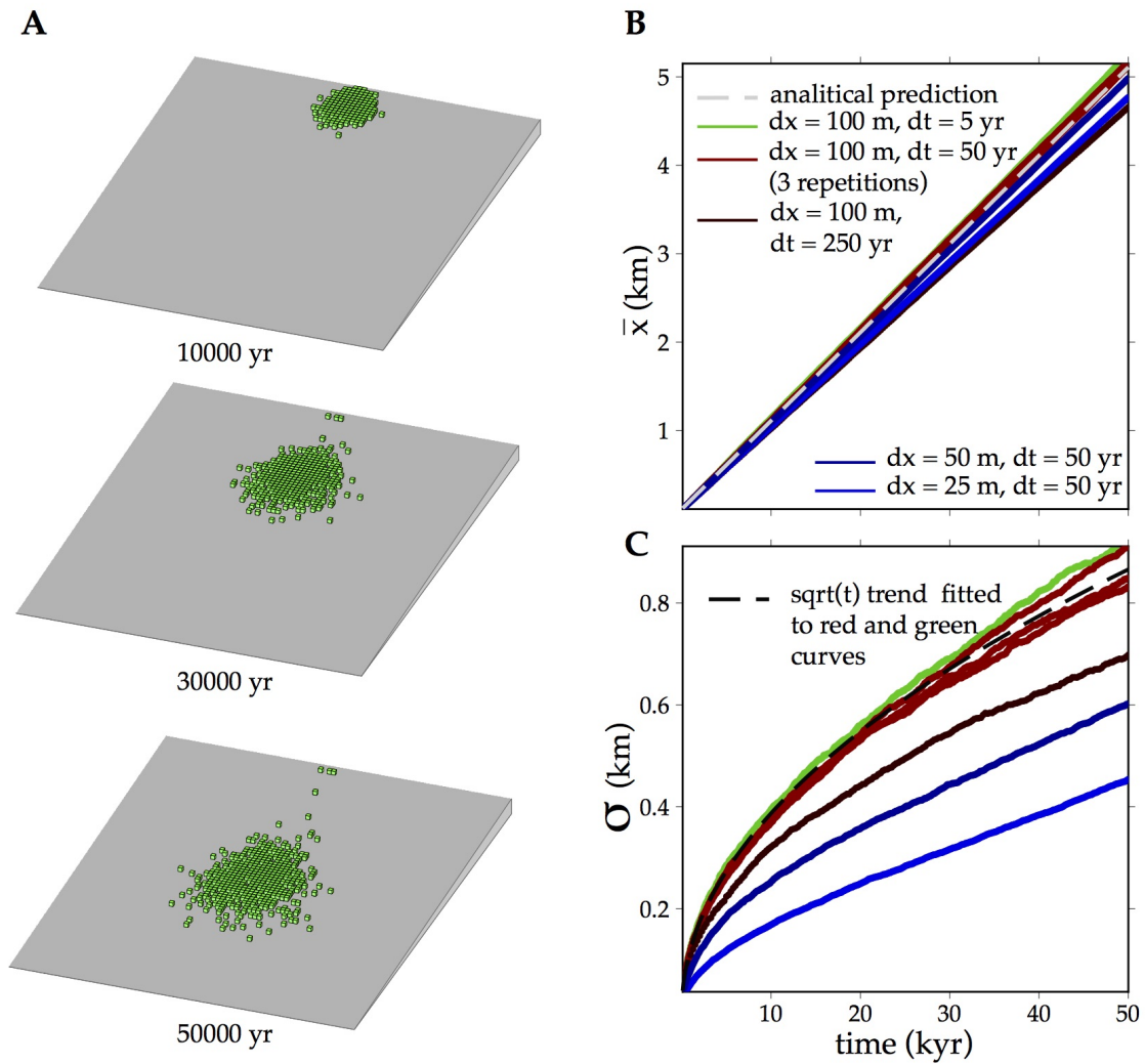
Figure 3. Model test in the linear diffusion case ( \epsilon = \kappa S and L = dx ). The initial plan slope is S = 0.1 . 1000 clasts are initially set at the surface and top of this plan. The diffusivity \kappa' = \kappa dx = 0.01 \text{ m}^2/\text{yr} in all the cases. A- Example of clasts spreading in the case \kappa = 0.0001 , dx = 100 \text{ m} and dt = 50 \text{ yr} . B- Evolution of the mean travel distances of the clasts for the different dx , dt and \kappa values. Note that the mean transport distance fits well with the prediction and does not significantly depend on dt or dx . C-Evolution of the standard deviation of the travel distances of the clasts \sigma . The black dashed curve is a \sqrt{t} fit to the reference (green-red) model curves, showing that \sigma \propto \sqrt{t} , consistently with the diffusion theory. Nevertheless, this fit overestimates by more than one order of magnitude the predicted curve ( \sigma = \sqrt{2\kappa dx t} ), which should correspond to a value of 0.036 km at t = 50 \text{ kyr} for the green and red curves.
