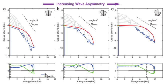
Figure 10. Plan views of modeled spits extending off of a headland eroding at a fixed rate of 0.08 \text{ m day}^{-1} after 137 model years (with “ghost” shorelines every 27 model years) above plots of normalized sediment transport and diffusivity. The only difference between simulations is the wave asymmetry (a) A = 0.5 , (b) A = 0.6 , and (c) A = 0.7 . Plot features explained further in Fig. 4 caption.
