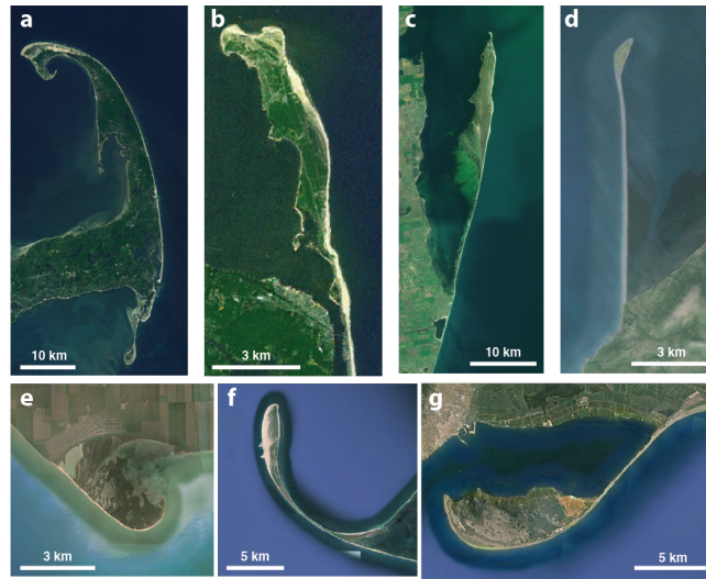
Figure 1. Natural examples of free spits: (a) Cape Cod, Massachusetts, USA, (b) Sandy Hook, New Jersey, USA, (c) Dzharylhach, Ukraine, (d) spit on Hagemester Island, Alaska, USA, (e) Kamyshevatskaya Spit, Russia, (f) Ostriv Tendrivs'ka Kosa, Ukraine, (g) La Banya Spit, Spain.
