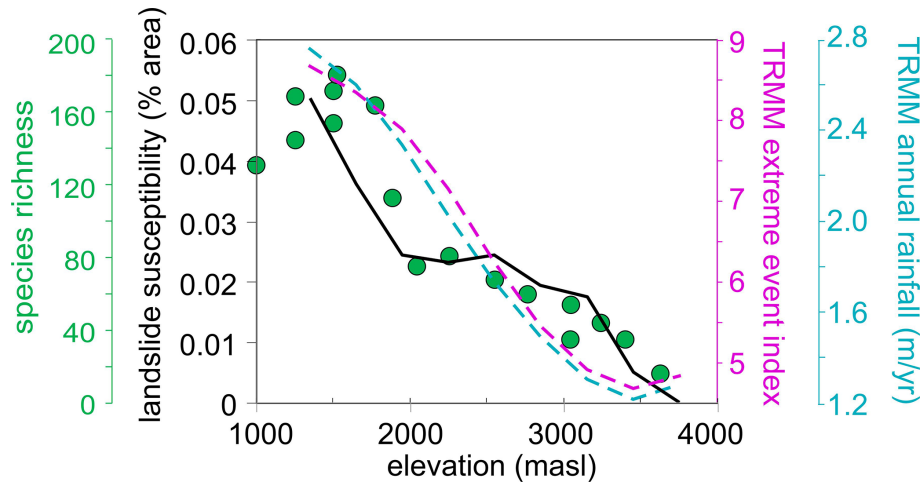
Figure 13. Plots of landslide susceptibility, TRMM-based precipitation (both total annual precipitation and TRMM extreme event index) (Bookhagen, 2013), and species richness, as a function of elevation within the Kosñipata Valley. Note that absolute values of 2B31 TRMM annual precipitation are not accurate without calibration to meteorological station data (cf. Clark et al., 2014) but spatial patterns may be representative. Climatology, landslide occurrence, and species richness all generally increase from high to low elevations within the Kosñipata Valley, although landslide susceptibility and species richness show a discontinuous trend with elevation while TRMM-based climatology is more continuous.
