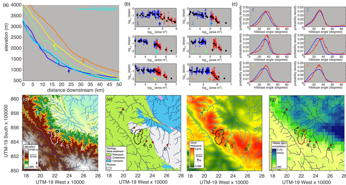
Figure 11. (a–c) Analysis of river profiles analogous to those in Fig. 10 (shown here as River #3, in cyan), for rivers throughout the Alto Madre de Dios region (d). In (b), data are binned by upstream area and means are shown by black circles. Arrows in (a) refer to locations along the profile of observed transition in the area-slope plots (b). These locations are displayed as red dots in (d–g), which show regional elevation (Farr et al., 2007) (d), geology (INGEMMET, 2013) (e), TRMM 2B31 annual precipitation (Bookhagen, 2013) (f), and Modis cloud frequency (Halladay et al., 2012) (g).
