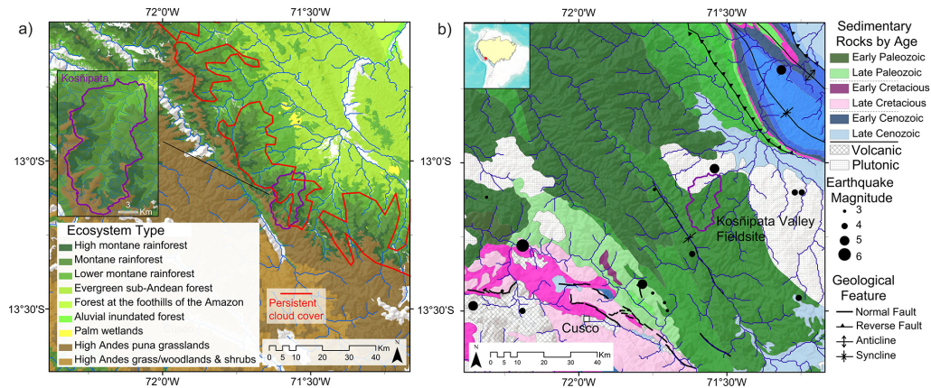
Figure 1. Maps of the study region. (a) Ecosystem types in the eastern Andes of Peru (Consió, 2011). Bare areas are cities, agriculture, glaciers and riverbed, with the Kosñipata study catchment magnified in the inset. Areas delimited by red polygons are regions of > 75% annual cloud cover (Halladay et al., 2012). (b) Georectified geological map (INGEMMET, 2013; Vargas Vilchez and Hipolito Romero, 1998; Carlotto Caillaux et al., 1996; Mendivil Echevarría and Dávila Manrique, 1994); sedimentary rocks are on a scale ranging from dark to light colour within each era. Active faults (Cabrera et al., 1991; Sébrier et al., 1985) and documented earthquakes since 1975 (USGS, 2013b) are shown.
