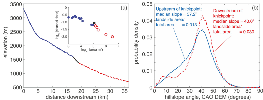
Figure 10. (a) Longitudinal profile along the Kosñipata river channel, with a prominent vertical step knickpoint evident between 1600 and 1400 m, corresponding to (inset) a transition in the plot between channel slope and upstream contributing area, calculated following Moon et al. (2011). (b) Probability density of hillslope angles (from 3 m × 3 m CAO DEM) upstream and downstream of the morphological transition in the channel, along with median hillslope angles in each region and landslide susceptibility over the 25 year study period.
