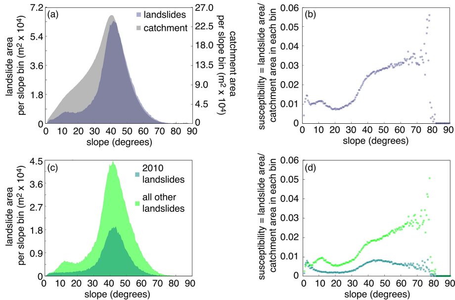
Figure 6. Histograms of catchment and landslide areas by slope bins of 1^\circ : (a) all landslides in the 25 year dataset; (c) separating landslides occurring during 2010, associated with the large storm in March 2010, from those in the rest of the dataset. (b) and (d) Corresponding calculation of landslide susceptibility, calculated as the area of landslides within each bin divided by the total visible area in the Landsat images used for mapping.
