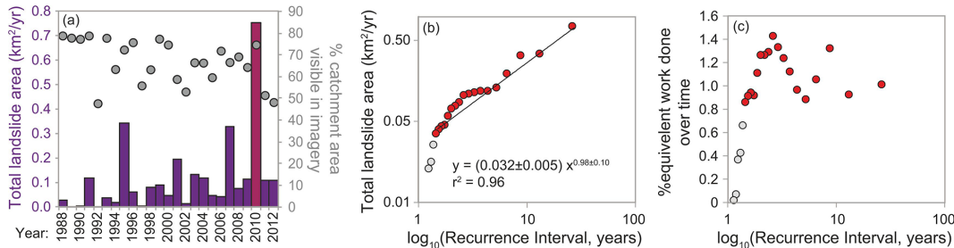
Figure 3. (a) Total area of landslides occurring each year in the dataset from this study, along with the % area visible in the images used for each year. (b) Magnitude–frequency relationship for landslide areas mapped in each year; red points are included in the regression while grey points are excluded since these lowest-magnitude years depart from the linear relationship. (c) Estimate of integrated work done by repeated events characteristic of given return times (see main text). Landslide area mapped in 2010 was significantly higher than any other year because of landslides triggered by the large storm in March 2010, but above a threshold magnitude, the integrated long-term landslide area triggered by repeated events of smaller magnitude is similar to that done by larger, rarer events in this dataset, as revealed by the similar % of equivalent work done for years across a wide range of inferred recurrence interval.
