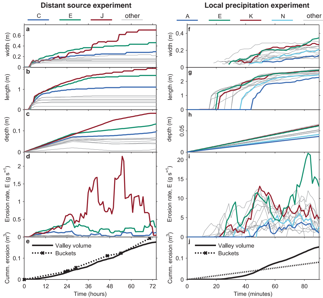
Figure 7. Valley development in the distal-distant source (left panel) and local precipitation (right panel) experiment experiments . Main valleys indicated with colors, letters in legend correspond with letters in Fig. Figure 5 . (a, f) (a, f) Valley width and (b, g) (b, g) length derived from orthorectified time-lapse imagery, (c, h) (c, h) valley depth derived from SFM-dems, (d, i) (d, i) estimated erosion rate from these properties and (e, j) (e, j) total cumulative erosion estimate from valley volume compared to measured sediment output.
