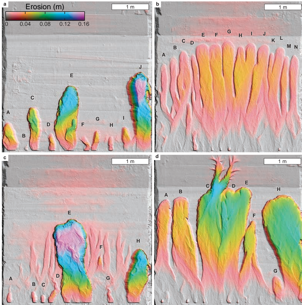
Figure 5. Erosion maps / final morphology of the experiments showing valley letters used in subsequent figures. (a) (a) Distant source experiment, (b) (b) Local precipitation experiment (c) (c) Distant after Local local and (d) (d) Local after Distant distant.
