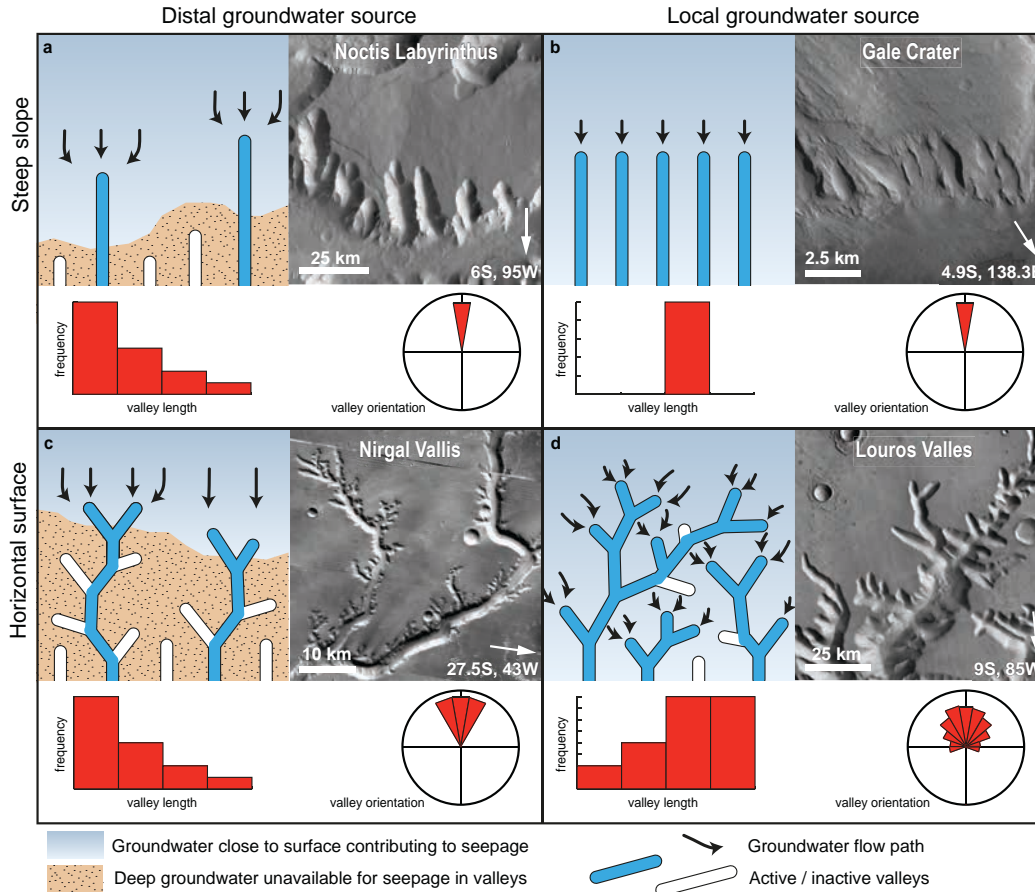
Figure 13. Landscape end-members formed by groundwater seepage as result from a distal distant source or local source precipitation , and steep or horizontal surface. Each panel shows a schematic schematic diagram (upper left), an Martian case showing a similar similar morphology (upper right) as an example and the expected valley length distribution and valley orientation (bottom). A distal distant source (a, c) (a, c) results in valley abandonment due to upstream capture of groundwater, where whereas a local local groundwater source (b, d) (b, d) is less prone to flow piracy. Horizontal surfaces (c, d) (c, d) have a strong strong tendency to form valley bifurcations in contrast to steep slopes (a, b) (a, b) . Distally fed valleys Valleys emerging from a distant groundwater source result in an open landscape as no valleys develop downstream of large valleys. Similar Martian landscapes in (a) (a) Noctis Labyrinthus (THEMIS image), (b) (b) Gale Crater (CTX image), (c) (c) Nirgal Vallis (THEMIS image) and (d) (d) Louros Valles (THEMIS image).
