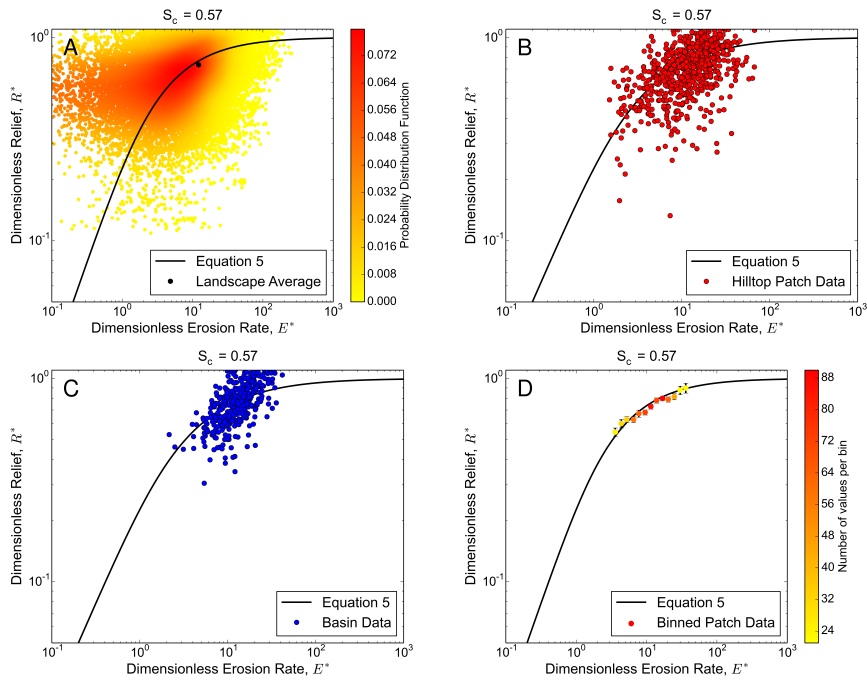
Figure 6. Comparison of the different methods which can be used to visualize E^* R^* from Coweeta, using a critical gradient of 0.57. (A) Raw data colored by the density of points in E^* R^* space alongside the landscape average value. Errorbars plot inside the data point. (B) Data averaged over hilltop patches. (C) Data averaged over second order drainage basins. (D) Hilltop patch data placed into logarithmically spaced bins, errorbars are the standard error.
