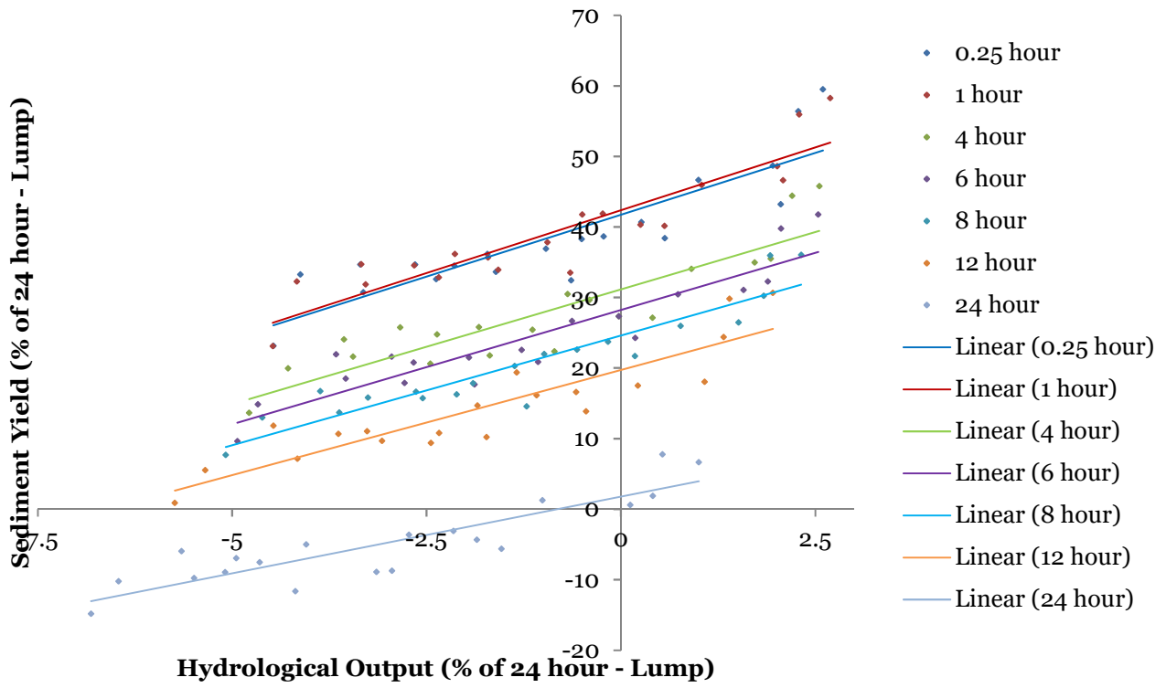
Figure 10. The relationship between hydrological output and sediment yield from each temporal resolution, based on outputs of the 20 jumble ensembles of the Upper Swale catchment.
