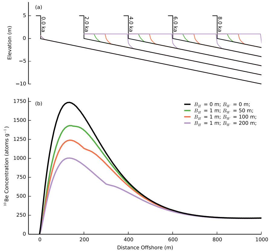
Figure 11. (a) Evolution of shore platform profiles over 10 ka with variable beach cover in the nearshore-near-shore described by a Bruun profile (Equation 6). Beach width reduces to B_w = 0 \text{ m} during the last 1000 yrs of the model runs. (b) Corresponding distribution of ^{10}\text{Be} for the case with no beach cover and thinning beaches during the last 100 yrs. The presence of beaches that disappeared over the last 1000 yrs would result in lower concentrations of ^{10}\text{Be} in the platform surface.
