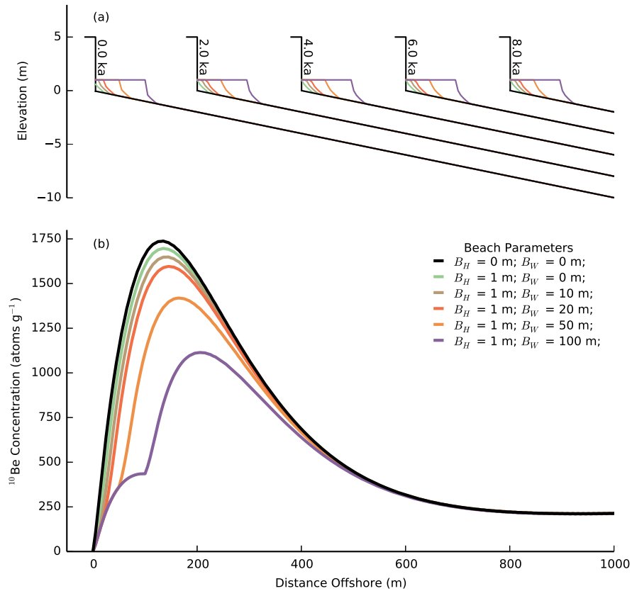
Figure 8. (a) Evolution of shore platform profiles over 10 ka with constant beach cover in the nearshore-near-shore described by a Bruun profile (Equation 6). (b) Corresponding distribution of ^{10}\text{Be} as a function of beach width. Beach cover reduces the concentrations of ^{10}\text{Be} in the platform surface, and wider beaches result in lower ^{10}\text{Be} concentrations and cause the position of the peak in concentrations to be further out from the cliff. Note that quite extreme beach cover B_W \geq 50 \text{ m} is required to significantly ( \geq 15\% ) reduce platform ^{10}\text{Be} concentrations.
