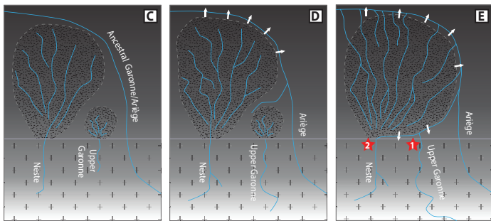
Figure 12: Comparison between (A) DEM of the Northern Pyrenees and foreland at the longitude of the Lannemezan megafan and (B) the final model (contour lines every 100 m) shown at the same scale. The proposed evolution for the Lannemezan megafan is schematized below: (C) A pre-existing river Ariège/lower Garonne River flows through the foreland while the Neste transports sediments deposited in the foreland through a distributive pattern to build a megafan; (D) a tributary of the Ariège/lower Garonne retreats headward and westward, towards the apex of the Lannemezan megafan while the megafan keeps growing; (E) the migration of the tributary leads to sequential capture of (1) the upper Garonne and (2) the upper Neste and thus the abandonment of the megafan; rivers incise together in the foreland deposit leaving a series of alluvial terraces (preferably on the left bank due to the direction of river migration indicated by white arrows).
