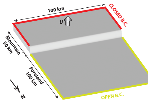
5 | Figure 2: The model grid consists of a mountain section, submitted to constant uplift U , and of a flat foreland section; both sections are submitted to precipitation. B.C. – Boundary Conditions; neither water nor sediment can cross a Closed B.C. while an Open B.C. corresponds to transverse rivers of fixed elevation capable of transporting both sediment and water fluxes out of the grid.
