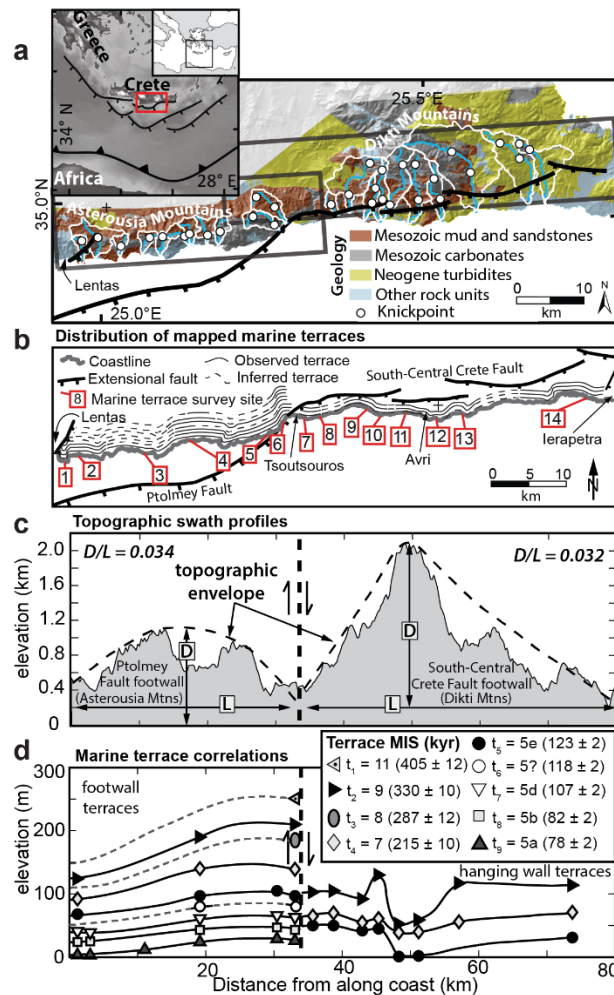
Figure 1: Inset maps show the location of the study area in south-central Crete and generalized tectonic setting. a. Digitized 1:50,000-scale geologic maps (Greek Institute of Geology and Mineral Exploration, 1972; 1974; 1977; 1987) with the outlines of the 21 drainage basins in thin white lines and trunk river channels in light blue. The dark gray rectangles show the locations of the elevation profiles shown in panel c. Active normal faults are shown as black lines with the hatch marks on the hanging wall after Gallen et al. (2014). b. Map of the south-central coastline of Crete with the geographic distribution of Pleistocene marine terraces. The figures are not drafted to scale, such that the vertical separation between terraces is relative. Sites 1 – 14 are the marine terrace survey sites from Gallen et al. (2014). The locations of some of the major towns and faults are shown. c. Maximum topography of south-central Crete as determined by swath profiles taken along the Asterousia and Dikti Mountains (see figure 1a for location). Dashed lines indicate the profile of maximum displacement as determined by correlation of the highest peaks in the respective fault blocks. The thick vertical dashed line indicates the location and sense of motion for an active extensional fault, the South-Central Crete fault. d. Terrace correlations for the south-central coastline of Crete (Gallen et al., 2014).
