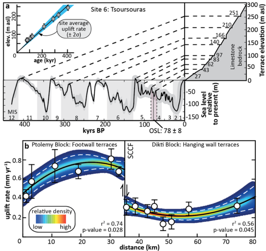
Figure 3: a. Correlation of the Tsoutsouras ( a – site 6; figure 1b) terrace sequences to the Late Quaternary global sea level curve (after Gallen et al., 2014). The 0 to 125 kyr sea level curve was compiled from Lambeck and Chappell (2001), while the 125 to 450 kyr segment is from Waelbroeck et al. (2002). Marine isotope stage (MIS) boundaries are from Lisiecki and Raymo (2005). Each terrace sequence is anchored to the sea level curve with an optically simulated luminescence (OSL) burial age of fine sand collected from marine terrace deposits. The Tsoutsouras sequence shows the OSL age of the lowest terrace in the sequence from Gallen et al. (2014). Inset diagrams show the total uplift versus estimated terrace age ( \pm 2\sigma ) and site average uplift rate from the Monte-Carlo regression analysis (dashed back line) with 2\sigma uncertainties (blue polygon). b. Site average uplift rates ( \pm 2\sigma ) are displayed as white circles. The coastal uplift model is shown as the black line and the white dashed lines depict the \pm 2\sigma uncertainties. The colored background shows the relative density of regression paths from the Monte-Carlo analysis. The location and sense of motion of the South-Central Crete fault (SCCF) is shown.
