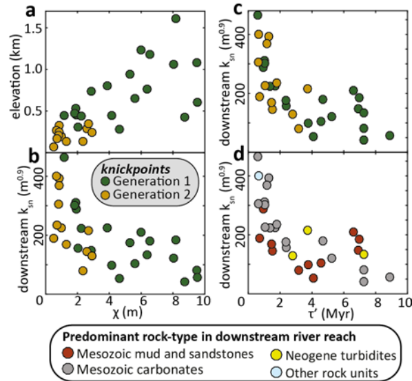
Figure 8: Plots of major knickpoint metrics from trunk channels in south-central Crete. a. \chi versus elevation for generation-1 and 2 knickpoints. The stream power incision model predicts knickpoints from a common origin will remain at the same \chi as they travel upstream provided that n = 1 and erodibility and drainage area are constant in space and time. b. \chi versus k_{sn} for generation-1 and 2 knickpoints. Note that for each generation there is an apparent weak inverse correlation between \chi and k_{sn} . c. \tau' versus k_{sn} for generation-1 and 2 knickpoints. d. same data as c, but each point is colored according to the predominant rock type on the next downstream reach.
