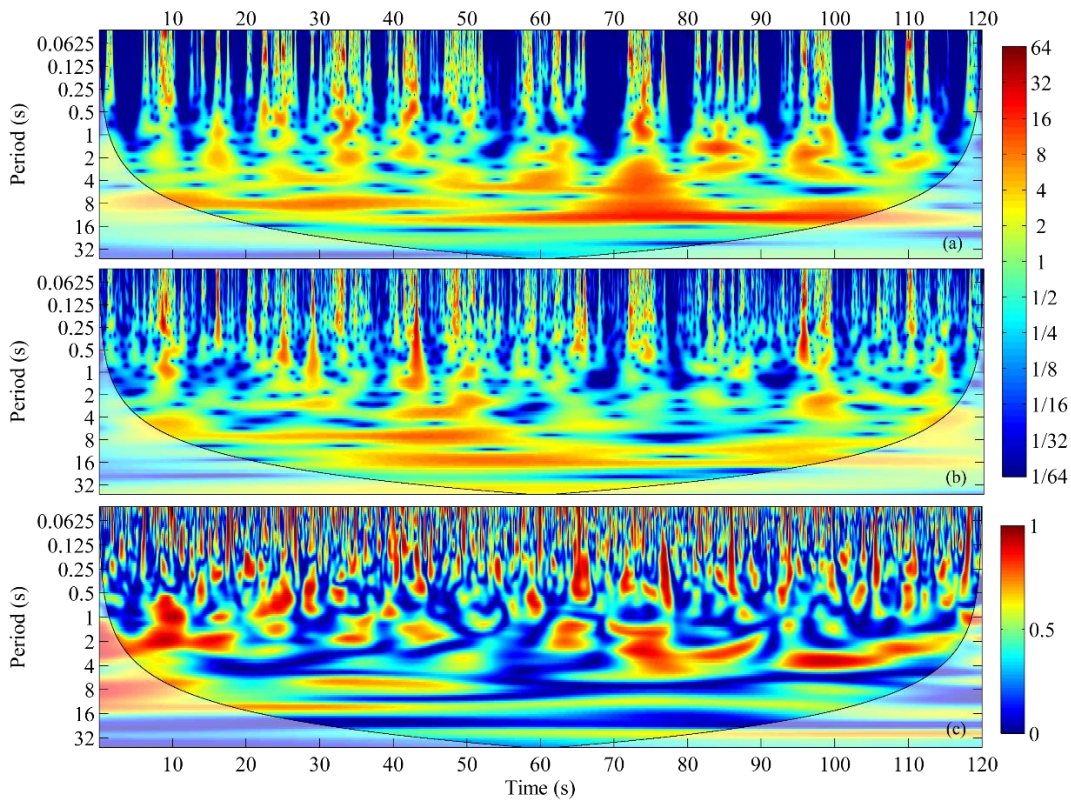
Figure 9. Wavelet power spectra (Morlet wavelet) for above the measured mean critical velocity experiment ( \bar{u} > \bar{u}_{cr, \text{measured}} ) for a two-minute period showing the (a) momentum flux ( u'w' ), (b) sediment flux ( c'w' ), and (c) coherence between the momentum and sediment fluxes.
