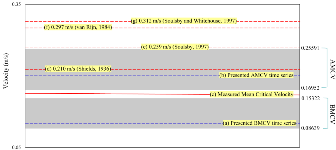
5 Figure 11. Schematic diagram showing the measured and calculated mean critical velocities.
