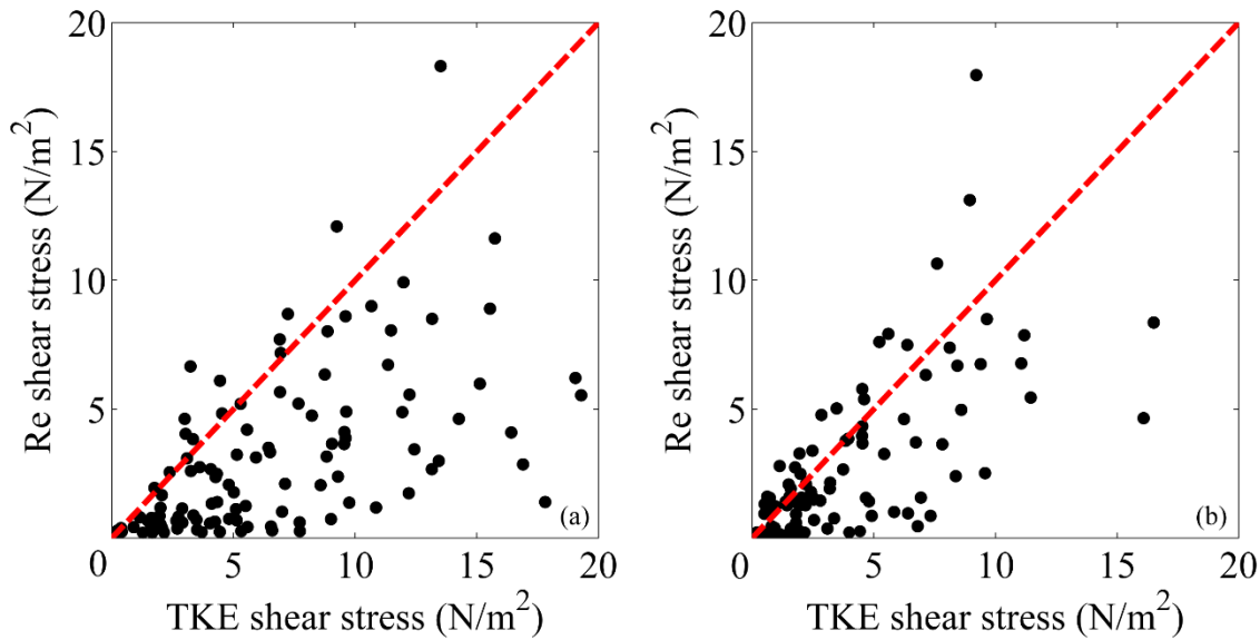
Figure 3. Comparison of the one-second mean Reynolds and TKE shear stresses from (a) above the measured mean critical velocity ( \bar{u} > \bar{u}_{cr, \text{measured}} ) and (b) below the measured mean critical velocity ( \bar{u} < \bar{u}_{cr, \text{measured}} ) experiments with a two-minute period. The dashed red line defines the equality.
