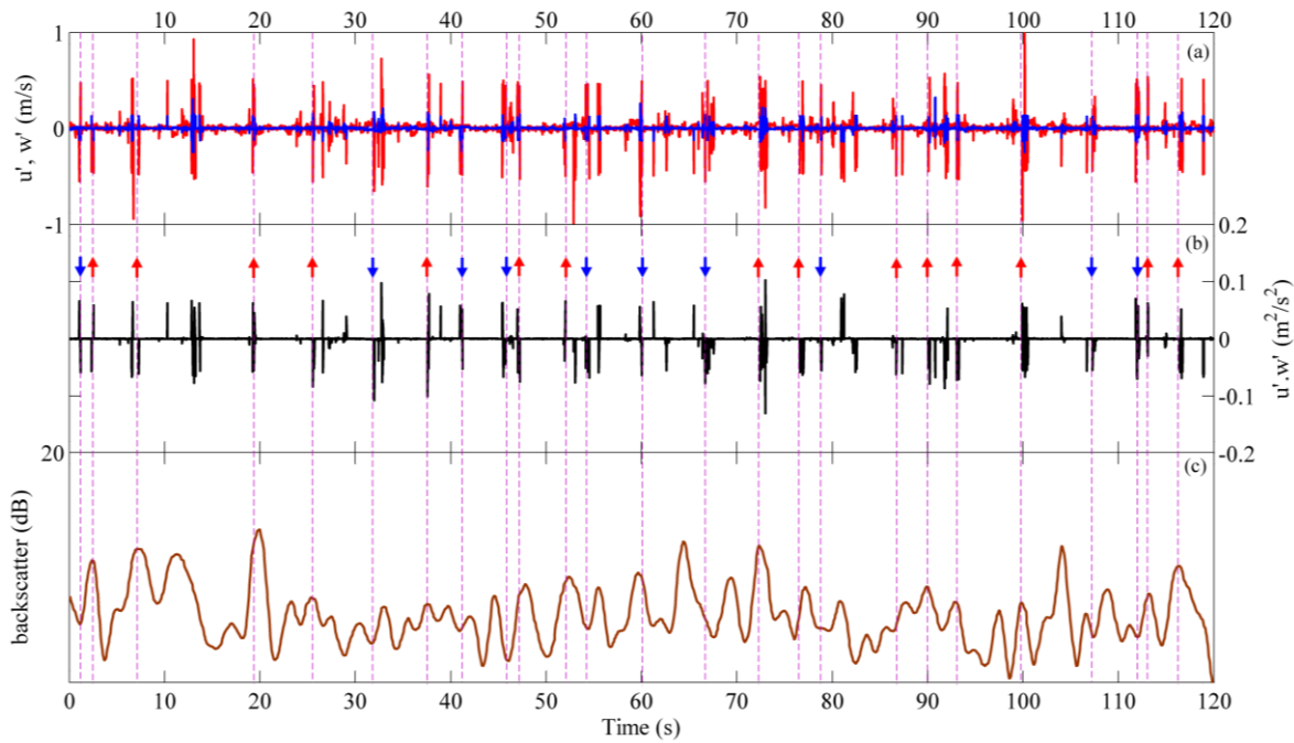
Figure 5. Time series records from below the measured mean critical velocity experiment ( \bar{u} < \bar{u}_{cr, \text{measured}} ): (a) turbulent velocity ( u' , w' ); (b) turbulent Reynolds shear stress ( u'w' ), showing the ejection (red up arrows) and sweep (blue down arrows) events; (c) one-second mean of the backscatter.
