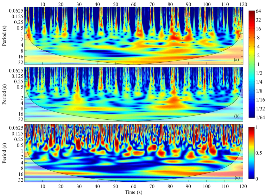
Figure 10. Wavelet power spectra (Morlet wavelet) for below the measured mean critical velocity experiment ( \bar{u} < \bar{u}_{cr, measured} ) for a two-minute period showing the (a) momentum flux ( u'w' ), (b) sediment flux ( c'w' ), and (c) coherence between the momentum and sediment fluxes.
