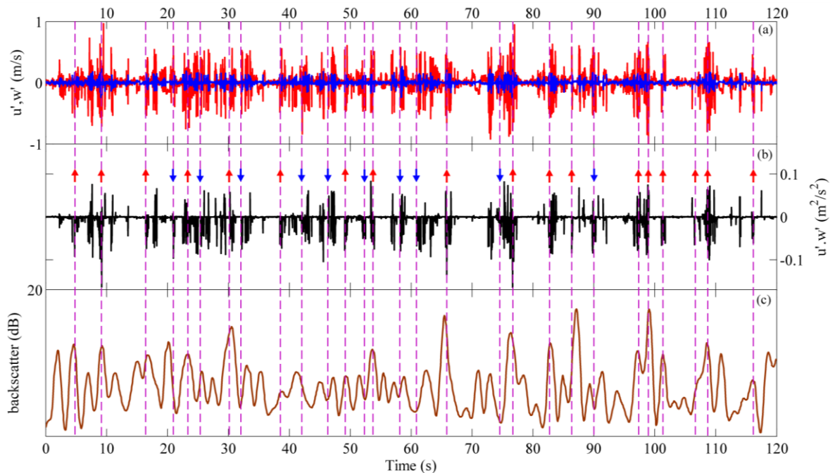
Figure 4. Time series records from the above measured mean critical velocity experiment ( \bar{u} > \bar{u}_{cr, \text{measured}} ): (a) turbulent velocity ( u' - red in color, w' - blue in color); (b) turbulent Reynolds shear stress ( u'w' ), showing the ejection (red up arrows) and sweep (blue down arrows) events; (c) one-second mean of the backscatter.
