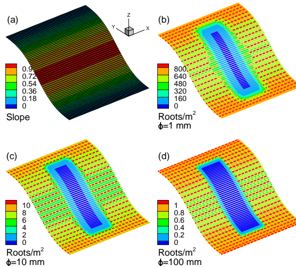
Figure 5. Tree-covered sigmoid slope, 70 \text{ m} \times 70 \text{ m} , with a 20 \text{ m} \times 50 \text{ m} clearing in its center. (a) Slope (unitless) with cell discretization (1 m). Density of roots crossing a vertical plane in units of roots \text{m}^{-2} for roots of diameter (b) 1 mm, (c) 10 mm, and (d) 100 mm.
