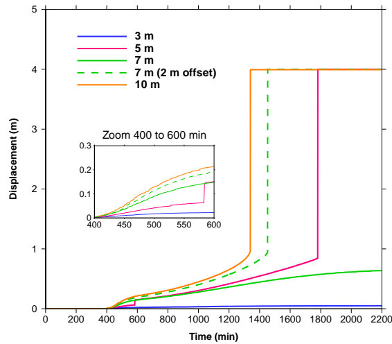
Figure 16. Effects of tree spacing on slope displacement at the center ( x = y = 0 ) for five different tree spacings and spatial configurations.
