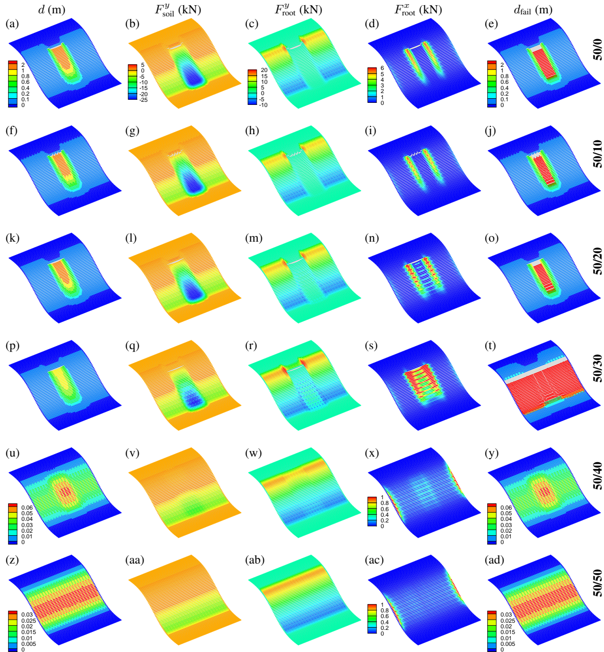
Figure 14. Effect of clearing tree size diameter on slope displacement and soil and root bond forces. From left to right, slope displacement ( d ), soil downslope compression ( F_{soil}^y ), downslope root force ( F_{root}^y ), and across-slope root force ( F_{root}^x ), at the time step just before failure and displacement at failure ( d_{fail} ) for the 6 simulations with different tree size diameters inside the clearing shown in Fig. 13. (a–e) Empty clearing (50/0), (f–j) DBH = 10 cm (50/10), (k–o) DBH = 20 cm (50/20), (p–t) DBH = 30 cm (50/30), (u–y) DBH = 40 cm (50/40), (z–ad) DBH = 50 cm (50/50). Outside the clearing, DBH = 50 cm. All trees are spaced 3 meters apart. Scale is given in the first row except when noted.
