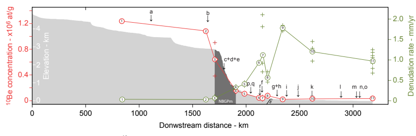
Figure 3: Downstream evolution of the 10 Be concentration (red) and corresponding denudation rates (green) of samples from the Tsangpo-Brahmaputra trunk stream. The elevation profile of the trunk stream channel is plotted in shaded grey. Down pointing arrows refer to the confluences with main Tsangpo-Brahmaputra tributaries. Open symbols are based on the average 10 Be concentration of all samples when multiple samples have been analyzed and crosses represent individual measurements. Open circles are from this study and open diamonds are samples from Finnegan et al. (2008).
