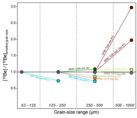
Figure 2: Ratio of 10 Be concentrations from grain-size pairs of a same sediment sample. Concentrations are normalized to the concentration of the lowest grain-size fraction for comparison amongst samples.
