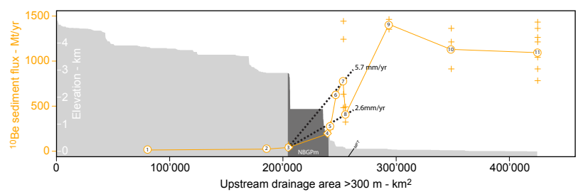
Figure 4: Evolution of the 10 Be-derived sediment flux as a function of the upstream drainage area above 300 m of elevation (in order to remove floodplain area storing sediments) from the Tsangpo-Brahmaputra trunk stream along with the channel elevation profile in grey. The average denudation rate over a given reach of the river is given by the slope of the regression between sample points. Open symbols are based on the average 10 Be concentration of all samples when multiple samples have been analyzed and crosses represent individual measurements. Open circles are from this study and open diamonds are samples from Finnegan et al. (2008).
