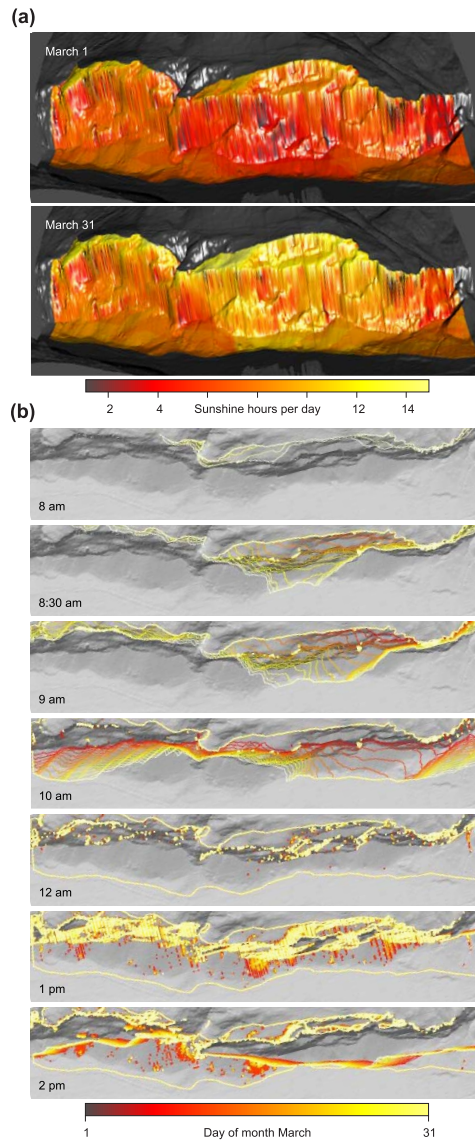
Figure 9. Potential sunshine coverage of the western Lauterbrunnen cliff face. a: Cumulative potential sunshine hours for the beginning and end of March 2015. The central part of the cliff shows the most changes, from 2–6 hours on 1 March to 6–14 hours at the end of this month. b: Sunlight-covered areas along the cliff face for different hours of the day (individual panels) and through the course of March 2015 (colour of the lines). The cliff cannot receive sunlight before 8 am, is completely in the sun by noon and in the shadow again around 1 pm. Again, the central cliff part is the most sensitive during 8 and 10 am. Sunlight polygons clipped to area of interest from figure 1.
