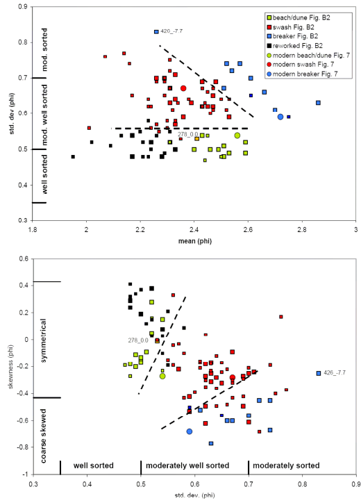
Fig. 3. Grain size statistical parameters, calculated conform the logarithmic method of moments (Blott and Pye, 1975).
