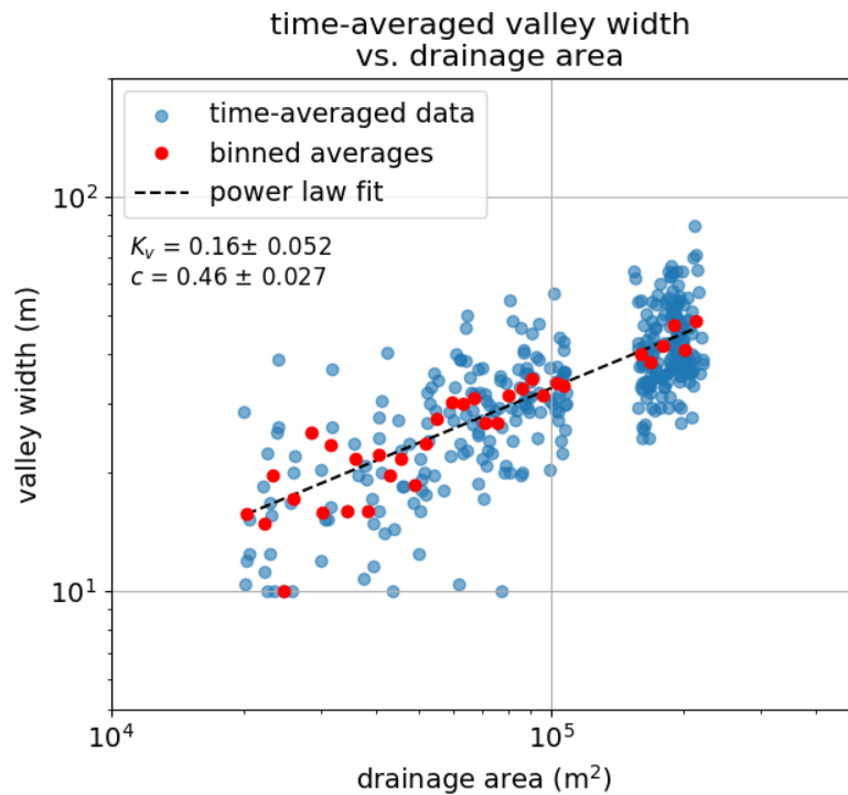
Figure 14. Valley width vs. drainage area for six time slices in the undercutting-slump, increased water flux model with dx=10 , K=10^{-4} , and \alpha=0.8 . All six time slices are from the model at steady state, with three time slices taken from the period of normal water flux and three time slices taken from the period of increased water flux. Each time slice represents data averaged over 2,500 years of model time, or 1.6% of the total length of the model run. Red dots show log-binned averages of valley width. The black line shows a least squares power law fit for the binned data. The K_v coefficient has a value of 0.16 with a standard error of 0.052 and the c exponent has a value of 0.46 with a standard error of 0.027.
