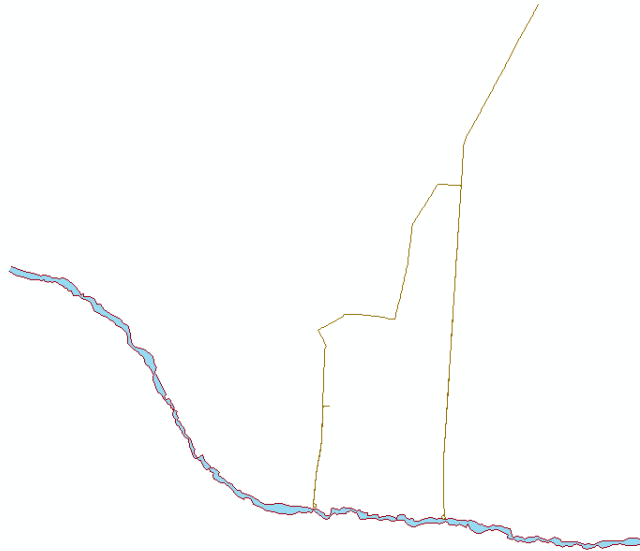
Figure 4: our given channel shape (red lines denote banks) and the resulting centerline (brown line) from the Planform Statistics Tool from the Toolbox Stream Restoration Toolbox
