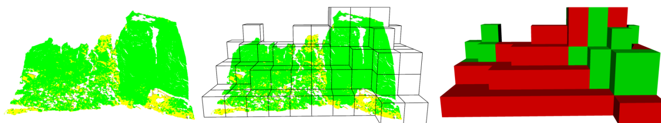
Figure 1: (Left) Binary inspection map of a test case. (Centre) Octree structure that contains the scene. (Right) Stable (green cubes) and unstable (red cubes) octree cells after congruence analysis.
