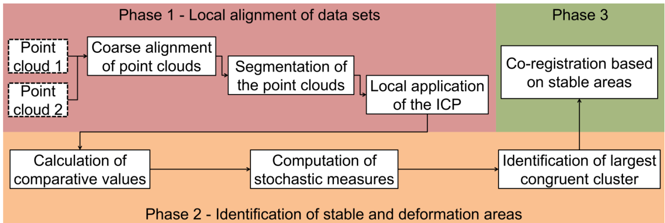
Figure 1: Workflow of the iterative closest proximity-algorithm (ICProx)
