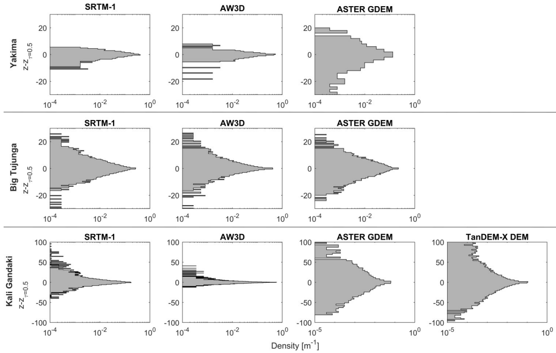
Fig. 7: Error distributions of longitudinal river profiles along the Yakima, Big Tujunga and Kali Gandaki calculated by the offset between measured elevations and elevations obtained with the CRS-algorithm with \tau = 0.5 and K = 5 .
