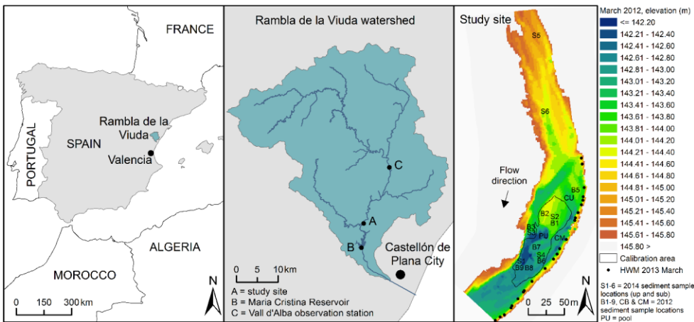
Figure 1: The study site of the Rambla de la Viuda, Eastern Spain. The elevation on March 2012 is derived mainly from mobile laser scanning data, but the edges are from the 2009 national digital elevation model. The calibration area was defined, based on the data coverage of March 2013. The high water mark (HWM) measurement locations of 2013 March are shown (their values are plotted in Fig. 3). Also the sediment sample locations are shown (see also Table 2 and Fig. 2).
