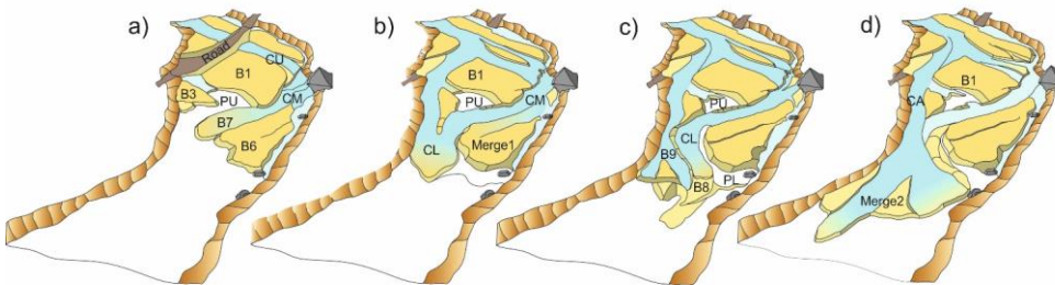
Figure 2: The conceptual graphic presented by Calle et al. (2015: Figure 10, www.schweizerbart.de/journals/zfg ): the pre-stage of 2012 (a), high flood stage during March 2013 event (b), low flow stage during May 2013 event (c) and final stage after May 2013 (d). CU: Upper Channel, CM: Middle Channel, CL: Lower Channel, PU: Upper Pool, PL: Lower Pool, B1-9: gravel Bars (cf. Calle et al., 2015).
