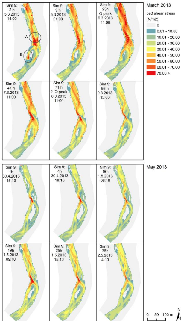
Figure 7: The bed shear stress of simulations 9 during moderate and small discharge events. The key time steps are presented (cf. Figure 5).
