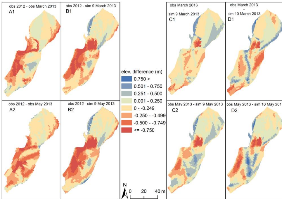
5 Figure 4: The comparison between the observed and simulated (simulations 9 and 10) elevations. The negative values (red) mean that the observed (A)/simulated (B: simulation 9) March (1)/May (2) 2013 topographies were higher (i.e. deposition had occurred) than was observed in 2012. The negative values also mean that simulated elevations of March/May 2013 were higher than was observed in March/May 2013 with simulations 9 (C) and 10 (D). Simulation 9 corresponded slightly better the observations than simulation 10, and thus its results are shown in more detail. The pool area, in the middle of the area, was the only area where simulation results clearly showed more deposition than observed (see also Fig. 2 PU). 10
