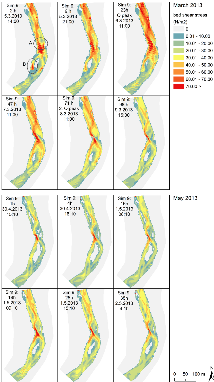
Figure 7: The bed shear stress of simulation 9 during moderate and small discharge events. The key time steps are presented (cf. Figure 5).
