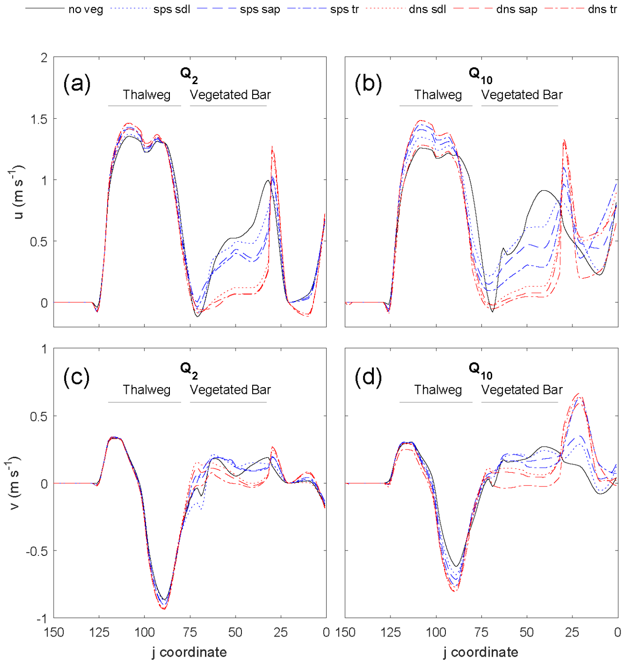
Figure 5. Effect of the vegetated bar ( j = 33\text{--}75 ) on the streamwise ( u ; a,b) and stream-normal ( v ; c,d) velocity at the downstream cross section (XS1) for the Q_2 (a,c) and Q_{10} (b,d) flows. With increasing discharge, plant size (seedling to young trees) and density, u
