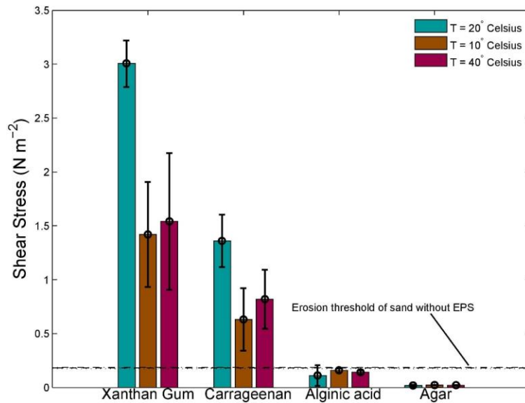
Figure 9. The erosion thresholds as a function of temperature for four synthetic extracted EPS as measured with the CSM erosion device. The horizontal lines correspond to the erosion thresholds of sand without EPS for a temperature of 20° Celsius (dashed), a temperature of 10° Celsius (dotted), and a temperature of 40° Celsius (dash-dotted). Error bars are standard deviation from n =3 repeat measurements.
