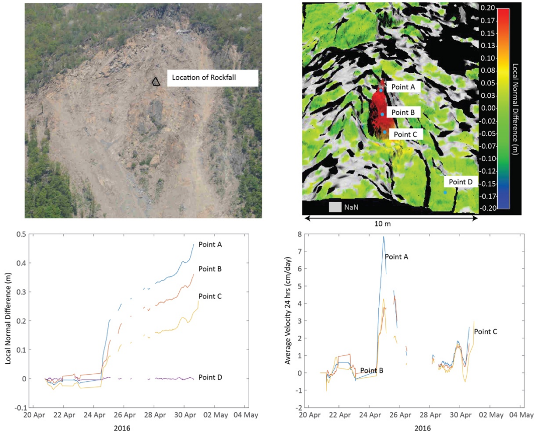
Figure 12: Pre-failure deformation of 80 m 3 rockfall. Top left, location of 80 m 3 rockfall. Top right, point cloud with mapped change showing deformation of the rock block prior to failure and 4 points used to plot time series data. Points A, B and C are located on the deforming area and Point D is located on an adjacent stable area of slope. Bottom left, deformation time series (cumulative values) of 3 points on the surface of the deforming rock block and a nearby stable point. Bottom right, average 24-hour velocity for Points A, B and C.
