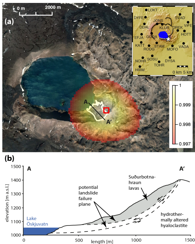
Figure 7: (a) Example of the tremor localisation results using the tremor record of the stations shown in the inset between 23:00:00 and 23:01:00 UTC, filtered between 1.5–3 Hz and a seismic wave velocity of 2300m/s. The open red square is the best-fit location and the ellipse around it is the likelihood quantile from 0.997 (red) to 1 (translucent white). The white line is the outline of the landslide source area. The inset shows the locations of the seismic stations used in the localisation and the location of the landslide source area (white star). (b) Hypothetical cross section of the landslide showing the potential stick-slip tremor planes.
