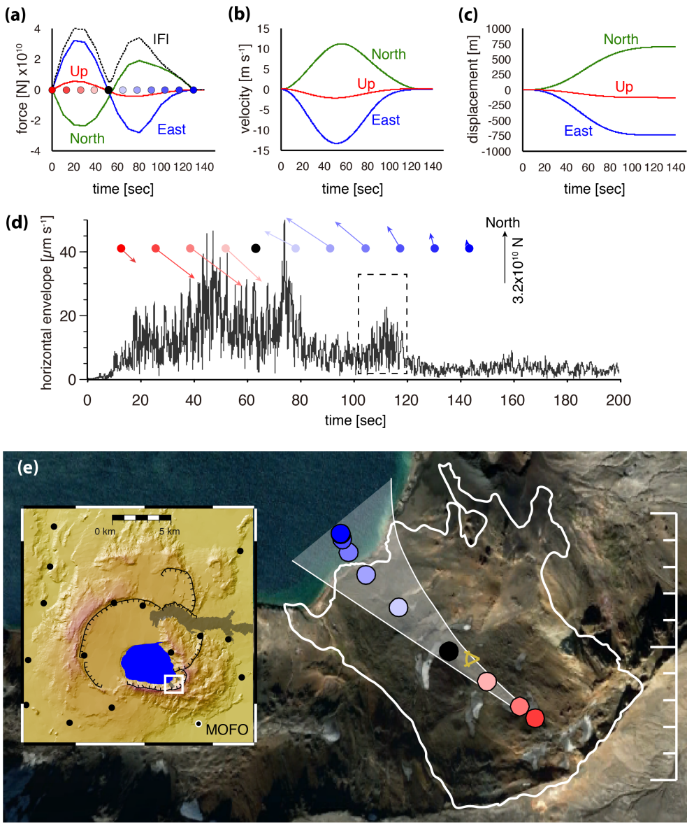
Figure 5: Results of the landslide force history inversion. (a) Force-time evolution, (b) velocity-time and (c) displacement-time plots for the north, east and upwards component of the loading force. Red circles in a), d) and e) mark the acceleration phase and the black circle is the transition to the deceleration phase (blue circles) of the landslide motion. (d) Time evolution of the landslide acceleration and deceleration with horizontal force vectors (arrows) for each time step (North is up). Horizontal envelope function of station MOFO (see inset in (e) for location), computed with the root-mean-square amplitudes of the horizontal component waveforms, filtered between 1–45 Hz for comparison. The dashed box highlights the late-arriving seismic signals. The start of the x-axis is at 23:24:05 UTC. (e) Path of the landslide bulk mass from the landslide force history inversion of the seismic waveforms between 0.02–0.08 Hz. Shaded white area is the range of the inversion results with different frequencies of the band pass filter (0.02–0.05 Hz, 0.02–0.08 Hz, 0.04–0.08 Hz). The white line is the outline of the landslide source area plotted on top of a Google Earth image taken on 7 August 2012. The yellow eye looking W is the location of the photography presented in Fig. 3. The white square on the inset shows the location of the main image.
