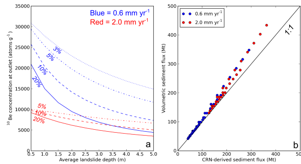
Figure 10. (a) Effect of event buffering on outlet \text{CRN-}^{10}\text{Be} concentrations, where smaller fractions (3, 5, 10 and 20%) of the event sediment are mixed into the fluvial network based on two background erosion rates of 0.6 and 2.0 \text{mm yr}^{-1} shown in blue and red, respectively. The event proportions are represented by the different dashed lines. The average landslide surface production-erosion rate is set to 3.0 \text{ mm yr}^{-1} , whilst the rest of the catchment is set to 35 \text{ atoms g}^{-1} . Under faster background erosion rates, the effect of larger landsliding events are more easily buffered in outlet \text{CRN-}^{10}\text{Be} concentrations. (b) Comparison of volumetric and CRN-derived sediment fluxes for event buffering scenarios. Under these conditions, volumetric and CRN-derived sediment flux estimates are much more comparable. In landscapes with lower background-erosion As the amount of landslide-derived material is mixed into the system increases, volumetric sediment fluxes are still become slightly larger with higher event inputs than CRN-derived sediment fluxes.
