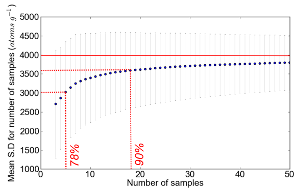
Figure 12. Number of 10 Be samples required to capture the natural concentration variability of the Ganga River. Approximately 18 samples are required to be within 10% of the true standard deviation (or variability) of the system. Blue dots represent the mean standard deviation of 100 populations of concentrations for a given sample group size (between 3 and 50). Error bars represent the standard deviation of the mean standard deviation of those 100 populations, per sample group size. The solid horizontal red line represents the mean standard deviation value that the sample group sizes converge towards (4,000 atoms g -1 ). The two dashed red lines represent the number of samples required to be within 10% of the true standard deviation (labelled 90%), and the standard deviation expected from a set of five samples (labelled 78%).
