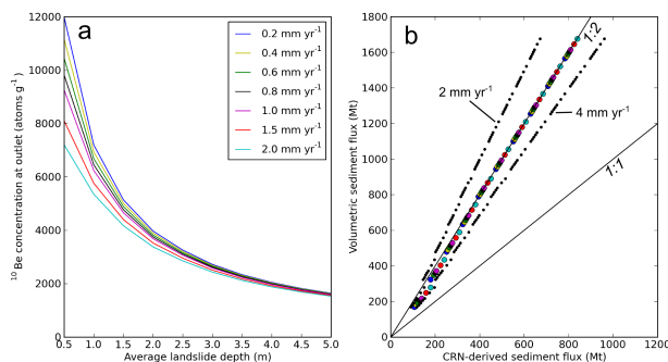
Figure 9. (a) Effect of lowering-increasing average landslide surface production-erosion rate to 10 atoms \text{g}^{-1} 3.0 \text{ mm yr}^{-1} on outlet CRN- ^{10}\text{Be} concentrations in response to varying landslide depths and catchment background erosion rates. The overall range in outlet concentrations is notably lower than in Fig. 8a. Increasing the catchment-averaged erosion rate only has an impact on outlet concentrations where the input of landslide material is smaller, suggesting that the outlet concentration is dominated by landslide-derived material. (b) Comparison of volumetric and CRN-derived sediment fluxes for the same model conditions, where marker colour corresponds to background erosion rate shown in part (a). The difference in volumetric and CRN-derived fluxes is much less than scenarios shown in Fig. 8d. In scenarios with higher background erosion rates general, the volumetric fluxes are only marginally higher than flux is approximately double the CRN-derived fluxes sediment flux. By increasing and decreasing the average landslide erosion rate to 4.0 and 2.0 \text{ mm yr}^{-1} as shown by the smaller black markers, this relationship varies slightly.
