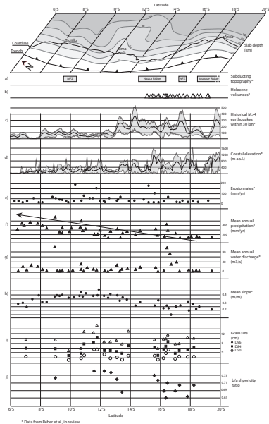
Figure 3. Topography of subducting Nazca plate, where slab depth data has been extracted from earthquake.usgs.gov/data/slab/. This N-S projection also illustrates: a) tectonic lineaments such as submarine ridges and MPZ, Mendocino Fracture Zone, NPZ, Nazca Fracture Zone; b) Holocene volcanoes; c) Earthquake data, taken from earthquake.usgs.gov/earthquakes/research/; number of earthquakes M w 4 within 30 km radius window; d) Coastal elevation. The data has been extracted from a 20 km wide swath profile along the coast. The three lines represent maximum, mean and minimum elevations within the selected swath; e) Catchment averaged denudation rates have been corrected for quartz content; f) Mean annual precipitation rates; g) Mean annual water discharge; h) Mean basin slope; i) Grain size results for the intermediate (b) axis of the pebbles in the streams from north to south at the sampling sites presented in Figure 1; j) Ratio between the intermediate axis and the long (a) axis (modified after Reber et al., in review).
