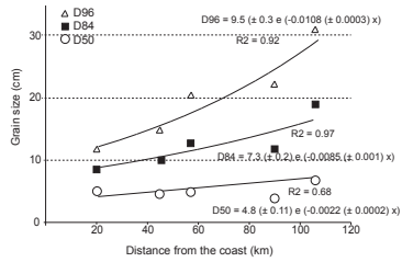
Figure 4: Grain size results along the Majes River.
