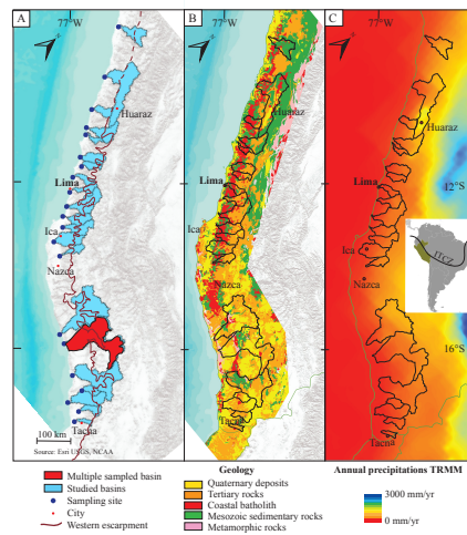
Figure 1: A: Map of the studied basins showing the sampling sites and the western escarpment (western escarpment modified after Trausestein et al., 2013). B: Geological map of the western Peruvian Andes. C: Map of the precipitation rates showing the spatial extend of the ITCZ, modified after Huffman et al., 2007.)
