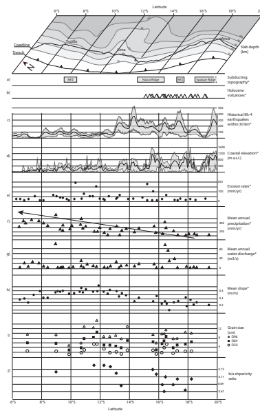
Figure 3: Topography of subducting Nazca plate, where slab depth data has been extracted from earthquake hypocenter data. This 3-D projection also illustrates: a) tectonic lineaments such as submarine ridges and MFZ; Mendocino Fracture Zone; MFZ; Nazca Fracture Zone; b) Holocene Volcanoes; c) Earthquake data. Taken from http://earthquake.usgs.gov/earthquakes/locate/ ; number of earthquakes M w 4.4 within 30 km radius window; d) Coastal elevation. The data has been extracted from a 30 km-wide mesh profile along the coast. The three lines represent maximum, mean and minimum elevations within the selected swath; e) Catchment averaged denudation rates have been corrected for quartz contents; f) Mean annual precipitation rates; g) Mean annual water discharge; h) Mean basin slope; i) Grain size results for the intermediate (b)-axis of the pebbles in the streams from north to south at the sampling sites presented in Figure 1; j) Ratio between the intermediate axis and the long (a)-axis (modified after Reber et al., in review).
