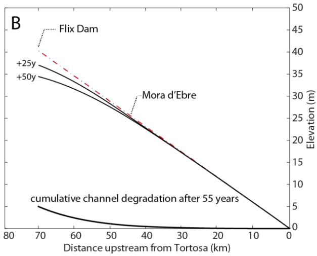
Figure 6. (A) A close-up of the Ebro drainage basin close to the delta (image Landsat). (B) Modeled response of the Ebro River downstream of the lowermost modern dam, the Flix dam.
