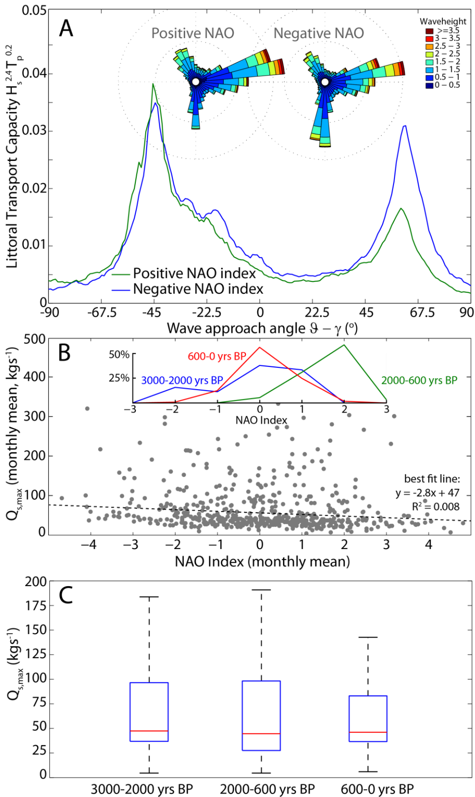
5 Figure 9. (A) The angular distribution of alongshore sediment transport potential from Hipocas hind-cast data (Sotillo et al., 2005), separated into periods of negative and positive monthly North Atlantic Oscillation (NAO) index (Jones et al., 1997). Insets show wave roses weighted by alongshore sediment transport potential for positive and negative NAO. (B) The monthly NAO versus the monthly maximum potential alongshore sediment transport Q_{s,max} . Dotted line shows the least-squares best fit line. Inset shows the NAO index distribution of Q_{s,max} for 3000-2000 years BP, 2000-600 years BP, and 600-0 years BP (Jones et al., 1997; Olsen et al., 2012). (C) Computed distribution of Q_{s,max} for different time periods.
