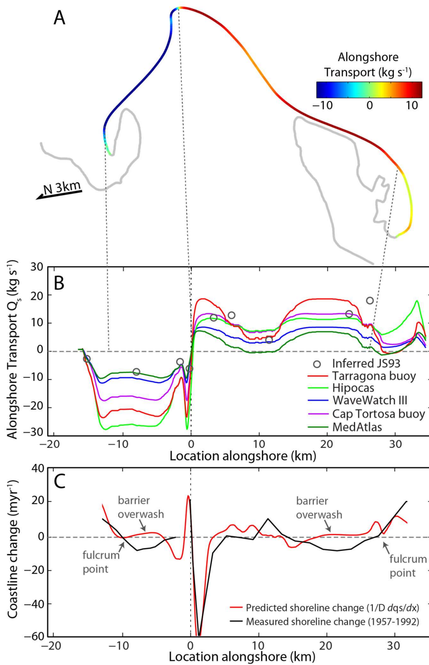
5 Figure 4. (A) The Ebro delta coastline, colored by the simulated alongshore sediment transport flux from the Cap Tortosa data. (B) Alongshore sediment transport along the Ebro delta coastline from all five wave climate sources (and assuming no sediment was supplied by the Ebro River). Alongshore transport is positive to the right when looking offshore. Black markers indicate alongshore sediment transport estimates from Jiménez and Sánchez-Arcilla (1993). (C) The Cap Tortosa buoy data recast into shoreline change rates using the one-contour-line approach (eq. 2) compared to the measured shoreline change rates from Jiménez and Sánchez-Arcilla (1993).
