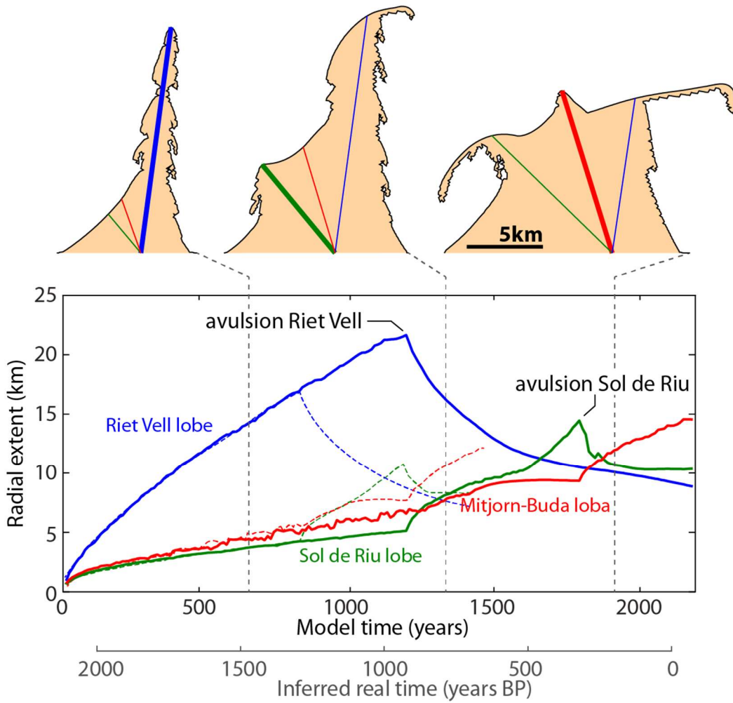
5 Figure 8. Simulated radial extent of the three different Ebro delta lobes for a sediment supply of 70 \text{ kg s}^{-1} and forced avulsions after 1200 and 1800 model years (solid lines) and after 800 and 1200 model years (dashed lines). Note that the radial extent can increase without the lobe being active because of littoral sediment transported from adjacent lobes. Three inset deltas show the solid line model run after 700, 1350 and 1900 years. The gray 2 nd horizontal axis indicates the real time inferred from the solid line model run and the modern Ebro delta morphology, where at the year 2015, lobes 1 and 2 are approximately 10 km long, and the active lobe is 15 km long, measured from the apex (Fig. 2).
