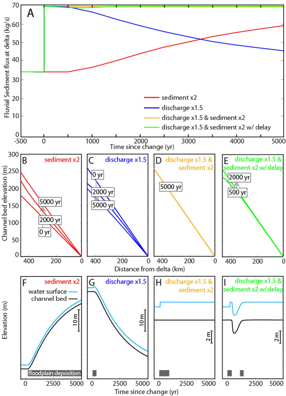
5 Figure 10. (A) Fluvial sediment flux at the apex of the delta and (B-E) longitudinal river profile evolution from four experiments of the river profile model with an increase in: sediment supply (red), flood discharge (blue), sediment supply and flood discharge (orange), and flood discharge with a lagged sediment supply (green). (F-I) Time evolution of the channel bed and water surface elevation through time, 200 km upstream of the delta at the approximate location of the floodplain records from Benito et al. (2008). Note the different scales between (F-G) and (H-I). Expected occurrence of floodplain deposits (period of increasing water surface elevation) shown by the grey bars.
