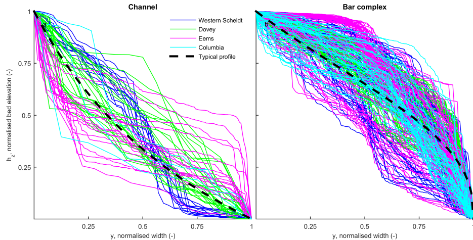
Figure 5. Hypsometric curves as extracted from bathymetry in the Western Scheldt, Dovey, Eems and Columbia River. Cross-sectional profiles were extracted along the centreline (Section 2.3) and were subsequently classified as channel when sand bars were (mostly) absent and as bar complex when one larger bar dissected by barb channels or multiple smaller bars were present. Channel-dominated morphology generally results in concave hypsometric profiles and bar complexes in convex profiles.
