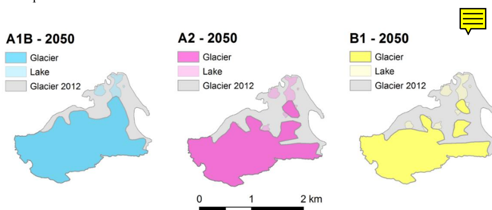
Figure 6. Modelled future glacier extent and possible areas for lake formation for the year 2050 under scenarios A1B, A2, and B1.
