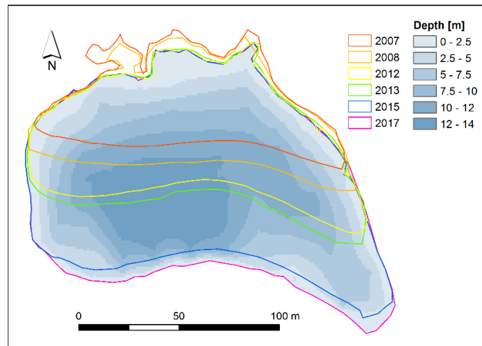
20 Figure 4. Bathymetric map and area changes of Lake 3 between 2007 and 2017. The lake depth data were gained during field survey carried out in 2017.
