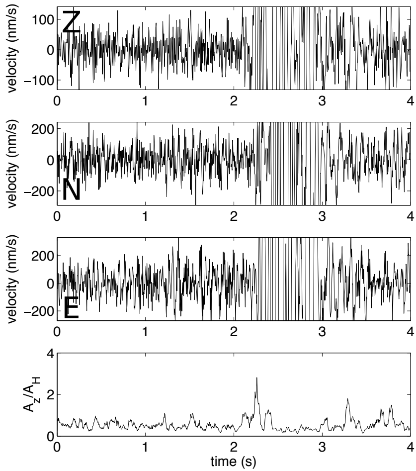
Figure 2: Same as Figure 1 for Seismic array B.
