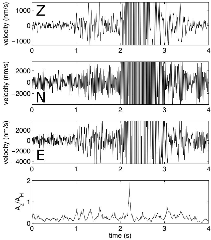
Figure 1: The three upper subplot display the Vertical and horizontal seismic traces for the Complex-Slopequake with precursor of the Super-Sauze landslide (12-Nov-2014 00:36:59, Seismic array A). The lower subplot shows the amplitude ratio between vertical and horizontal traces. The precursor signals are starting approximately at 1s.
