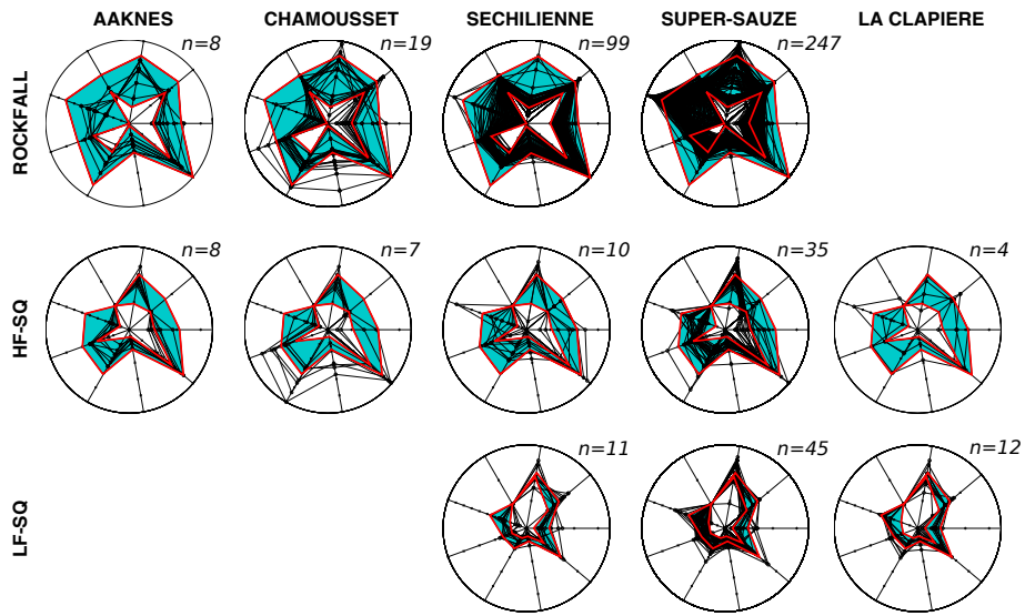
Figure 12. Variability of the signal features of classes “Rockfall”, “HF-slopequake” and “LF-slopequake” for five different sites: Aaknes, Chamousset, Séchilienne, Super-Sauze and La Clapière. The axes of the star diagram are the same as in Fig. 11.
