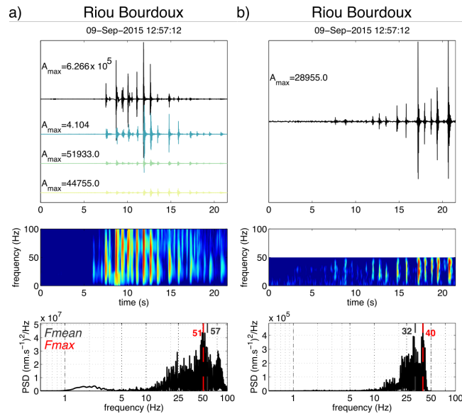
Figure 2. Example of one controlled rockfall (mass= 430kg) at the Riou-Bourdoux catchment (Hibert et al., 2017a) recorded by SP seismometer located at 50 m of the rock departure (left) and recorded by BB seismometer near the rock arrival (right). The waveforms of the vertical traces are plotted on the upper part of the figure. The amplitude are normalized on the trace with the maximal amplitude (black), the signal recorded by the other sensors (when available) are represented in color below. The maximal amplitudes ( A_{max} ) of all the traces are plotted on the sub-plot. The spectrogram is plotted on the middle part of the figure and normalized to the maximal energy. The lower part of the figure represents the PSD of the most energetic trace and the frequency corresponding to the maximum and the mean of the PSD are plotted in red and gray respectively.
