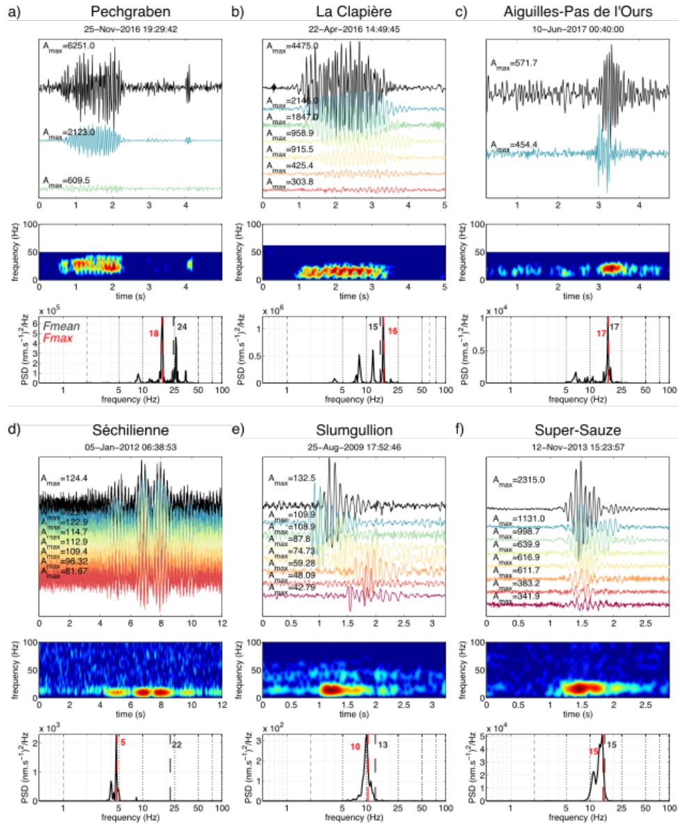
Figure 13. Examples of pure harmonic signals recorded at the a) Pechgraben, b) La Clapière and c) Aiguilles-Pas de l'Ours, d) Séchilienne, e) Slumgullion (Gomberg et al., 2011) and f) Super-Sauze slopes. See Fig 2 for description of the figure.
