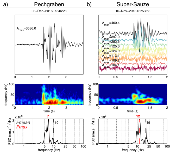
Figure 8. Hybrid-Slopequake recorded at the a) Pechgraben and b) Super-Sauze landslide. See Fig 2 for description of the figure.
