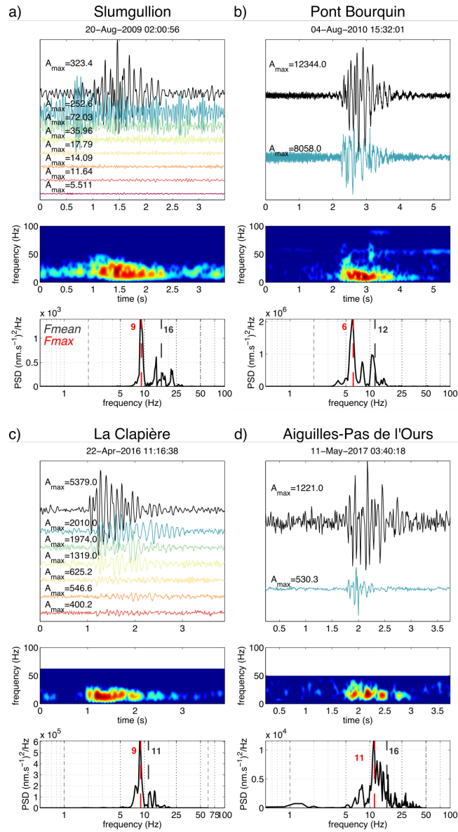
Figure 6. Low-Frequency Slopequakes recorded at the a) Slumgullion (Gomberg et al., 2011), b) Pont-Bourquin, c) La Clapière and d) Aiguilles-Pas de l'Ours slopes. See Fig 2 for description of the figure.
