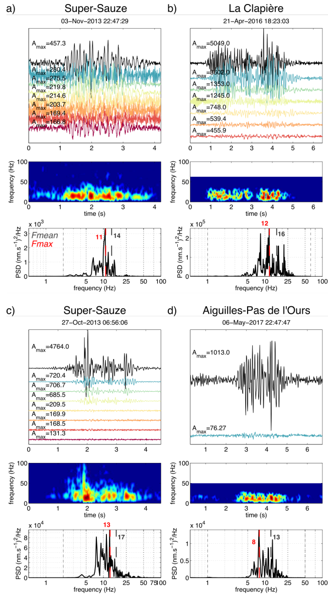
Figure 10. Examples of repetitive Slopequakes recorded at the a),c) Super-Sauze, b) La Clapière and d) Aiguilles-Pas de l'Ours slopes. See Fig 2 for description of the figure.
