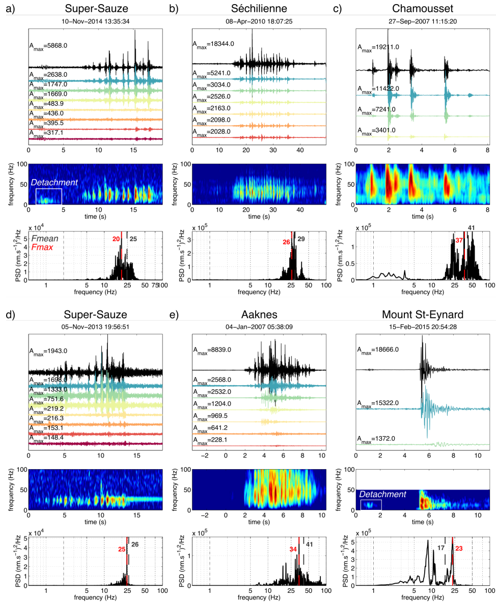
Figure 3. Rockfall events recorded at a) and d) Super-Sauze (France) (Provost et al., 2017a), b) at the Séchilienne (France, Helmstetter et al. (2011); RESIF/OMIV (2015)), c) Chamousset (Levy et al., 2011), e) Aaknes and f) Mount Saint-Eynard slopes (Le Roy et al., 2018). See Fig 2 for description of the figure.
