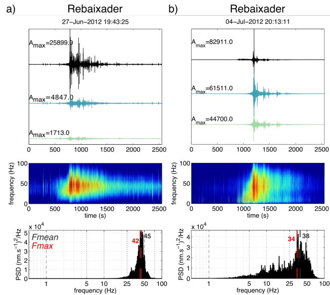
Figure 5. Wet granular flow events recorded at Rebaixader torrent (Abancó et al., 2012; Hürlimann et al., 2014; Arattano et al., 2016). See Fig 2 for description of the figure.
