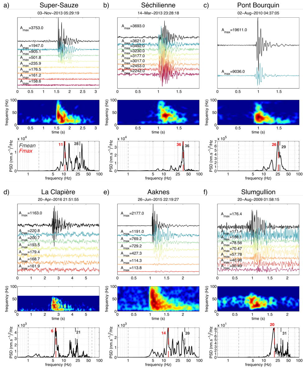
Figure 7. High-Frequency Slopequakes recorded at the a) Super-Sauze (Provost et al., 2017a), b) Séchilienne (Helmstetter et al., 2011; RE-SIF/OMIV, 2015), c) Pont-Bourquin, d) La Clapière, e) Aaknes, and f) Slumgullion (Gomberg et al., 2011) slopes. See Fig 2 for description of the figure.
