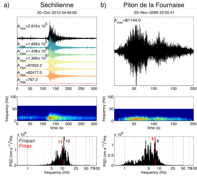
Figure 4. Dry granular flow events recorded at a) Séchilienne and b) the Piton de la Fournaise Caldera. See Fig 2 for description of the figure.
