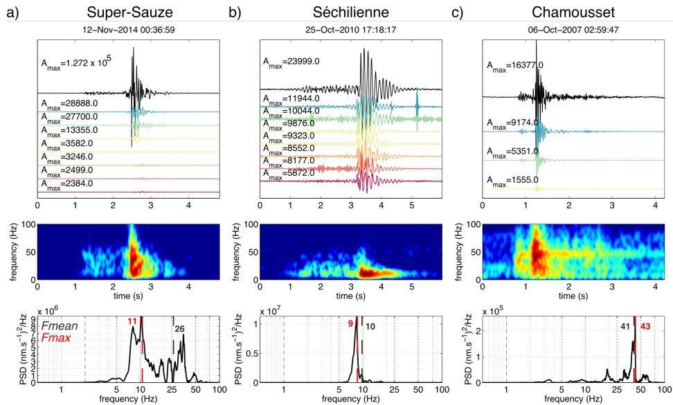
Figure 9. Examples of Slopequakes with presursory event recorded at the a) Super-Sauze, b) Séchilienne and c) Chamousset slopes. See Fig 2 for description of the figure.
