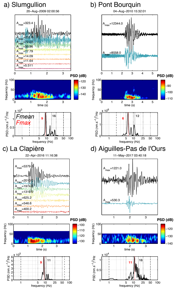
Figure 6. Low-Frequency Slopequakes recorded at the a) Slumgullion (Gomberg et al., 2011), b) Pont-Bourquin, c) La Clapière and d) Aiguilles-Pas de l'Ours slopes. See Fig. 2 for description of the figure. Note that for the Slumgullion signals (a), the amplitudes are expressed in counts.
