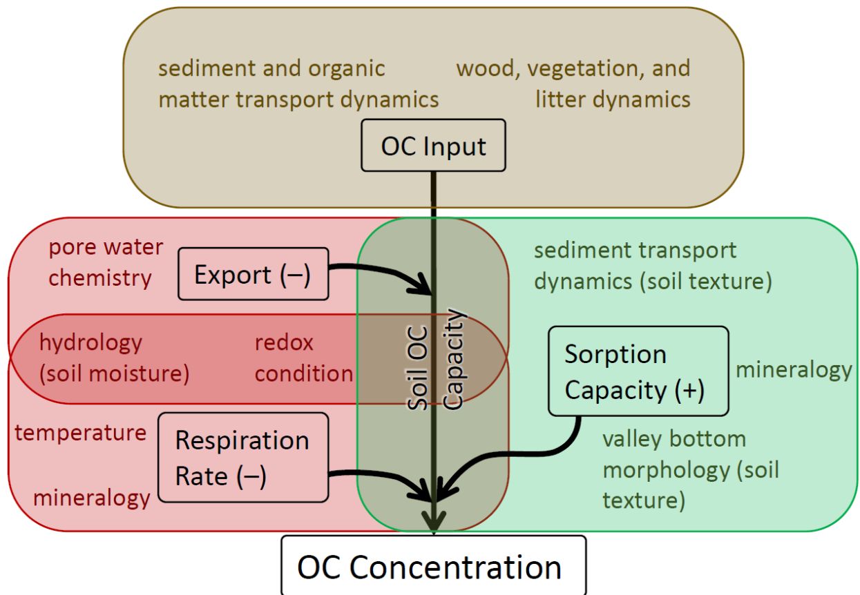
Figure 4: Conceptual model of physical processes that influence OC concentration in floodplain soils, based on this study and other literature. Each box corresponds to a major factor that influences OC concentration. Colored text within each box denotes factors that influence OC inputs, sorption capacity, OC export, or respiration rate (note that some processes influence both OC export and respiration rate). As sorption capacity increases, so does the OC capacity of the soil. Conversely, as the rate of respiration and/or OC export increases, the soil OC capacity decreases. Floodplain soils can only develop high concentrations of OC if there are high rates of OC input. However, the capacity of the soils to store OC regulates that input, and is determined by the competing influences of sorption capacity and the combination of respiration rate and OC export. See text for further details.
