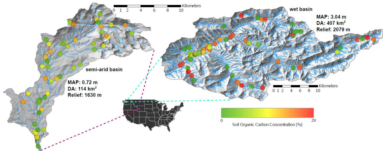
Figure 1: Hillshade showing the location, sampling sites, and stream network of the sampled basins. Big Sandy, Wyoming ( 42.69^{\circ} , -109.25^{\circ} ), on left and MF Snoqualmie, Washington ( 47.53^{\circ} , -121.52^{\circ} ), on right. Circles represent sampling locations at which floodplain soil OC was measured. Sample sites are colored by OC concentration. Mean annual precipitation (MAP), drainage area (DA), and relief are given for each basin.
