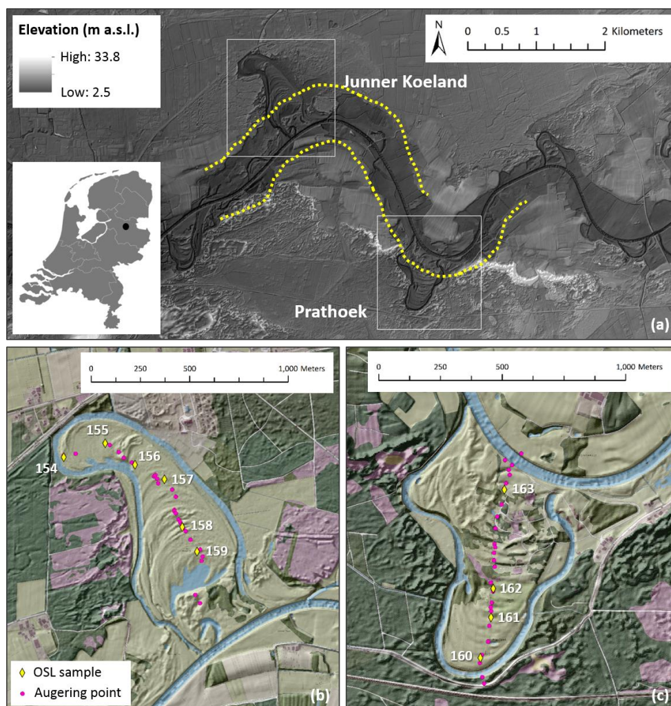
Figure 1. Location of the study area (a), showing the two meander bends Junner Koeland (b) and Prathoek (c). Dotted line in (a) indicates the valley edge. M a.s.l. = metres above sea level. White numbers along the coring transects in (b) and (c) indicate OSL sample locations by abbreviated sample code (all should be preceded by NCL-2415). Samples NCL-2415154–162 were collected in point bar deposits, sample NCL-2415163 was collected in a terrace remnant. Lithological cross sections and lithogenetic interpretation are provided in Candel et al. (submitted). Digital elevation model (AHN2, horizontal resolution 5 m, vertical resolution 0.2 m): AHN (2018); Van Heerd and Van't Zand, (1999). Topography (3200 pixels/km): OpenTopo, Van Aalst (2017).
