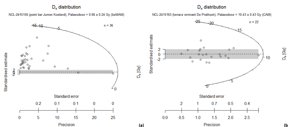
Figure 6. Two radial plot examples showing (a) a point bar sample (NCL-2415156) from Junner Koeland, and (b) the sample collected in a terrace remnant near Prathoek (NCL-2415163). The point bar sample in (a) is poorly bleached, showing a large population of grains with a D_e of about 10 Gy. Such equivalent doses are similar to those of the terrace sample in (b) (CAM: D_e 10.43 ± 0.43 Gy).
