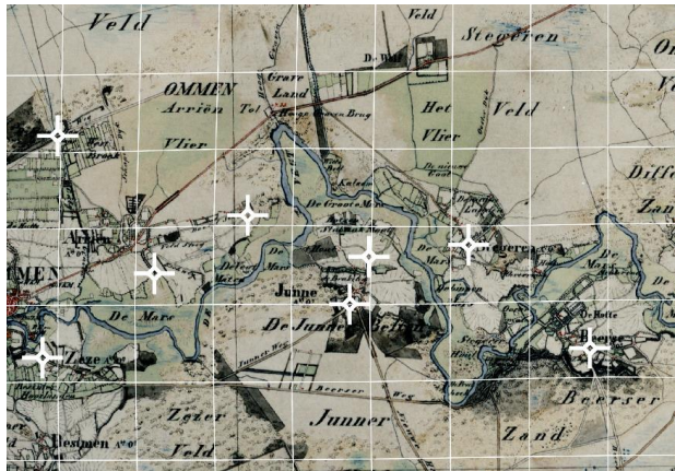
375 Figure 4. Fragment of the georeferenced historical map of 1851 AD (details listed in Table 2), displaying ground control points (white plusses) and a distortion grid (in white, maze size of 1 km). The grid approaches a perfect grid, indicating that map distortion is minimal. Grid generated with MapAnalyst software by Jenny and Hurni (2011). Image reference historical map: CC-BY Kadaster, 2018.
