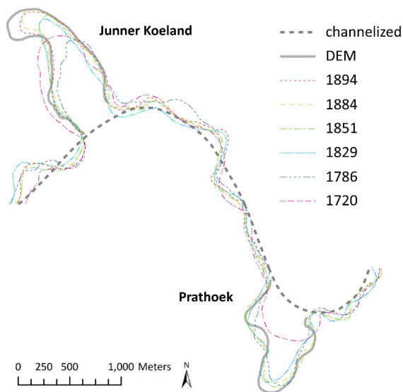
380 Figure 5. Channel centrelines as derived from the historical maps (years AD) listed in Table 1 and shown in Fig. 2. The DEM (digital elevation model) line represents the course of the meanders preserved upon abandonment at the time of channelization (between 1884-1901 AD for Prathoek and between 1894-1906 AD for Junner Koeland).
