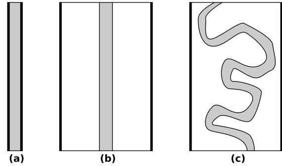
Figure B1. Our equations for sediment transport follow the river, but geomorphic evolution occurs along valley networks. In some cases (a), these are perfectly aligned and have the same width. However, if the river is aggrading and the valley walls are not vertical, and/or the river is eroding its valley walls at a rate that is comparable to or faster than its rate of vertical incision, (b) the river may carve a valley that is wider than its channel. (Here, the channel is pictured in the center, but it need not be positioned there.) In creating a wide valley, the river may move laterally, leading to (c) downstream and down-valley flow directions that are not aligned. While this depicts a single-thread channel, this same differentiation between channels and valleys is applicable to multi-thread channels.
