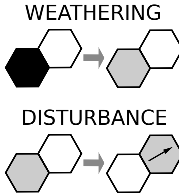
Figure 7. Transitions representing rock-to-regolith transformation by weathering (top), and regolith disturbance (bottom), in which a stationary particle becomes mobile and switches position with an air cell. Illustration represents one of the six possible orientations.
