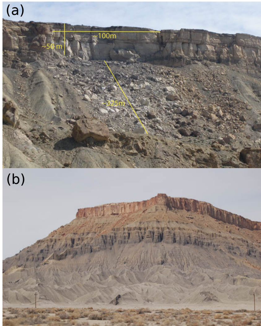
Figure 15. Two examples of cliff-and-rampart morphology. (a) Near Palisade, Colorado, USA, after recent rock-fall event (photo courtesy D.N. Bradley and D. Ward). (b) Colorado Plateau, Utah, USA. Note that contact between lower rampart and sub-vertical slopes, both of which have formed in a gray shale unit, occurs without any apparent break in lithology.
