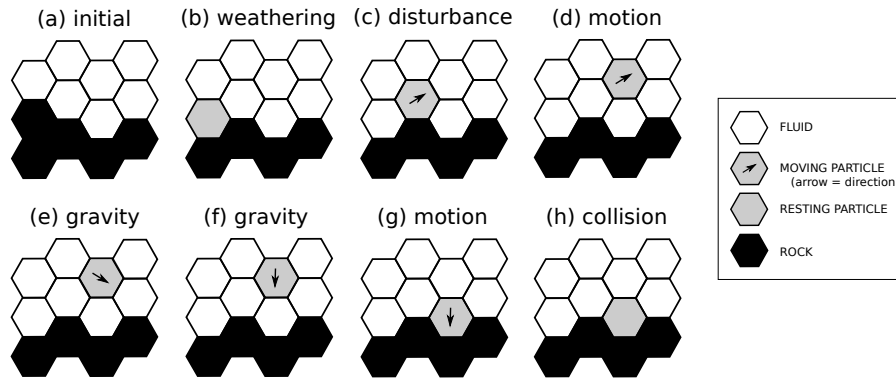
Figure 3. Hypothetical time sequence of transition events, from upper left to lower right, illustrating several of the states and transitions in the Grain Hill model. Note that although this example shows a single particle in motion, it is possible for multiple cells to exist in a state of motion at any given time.
