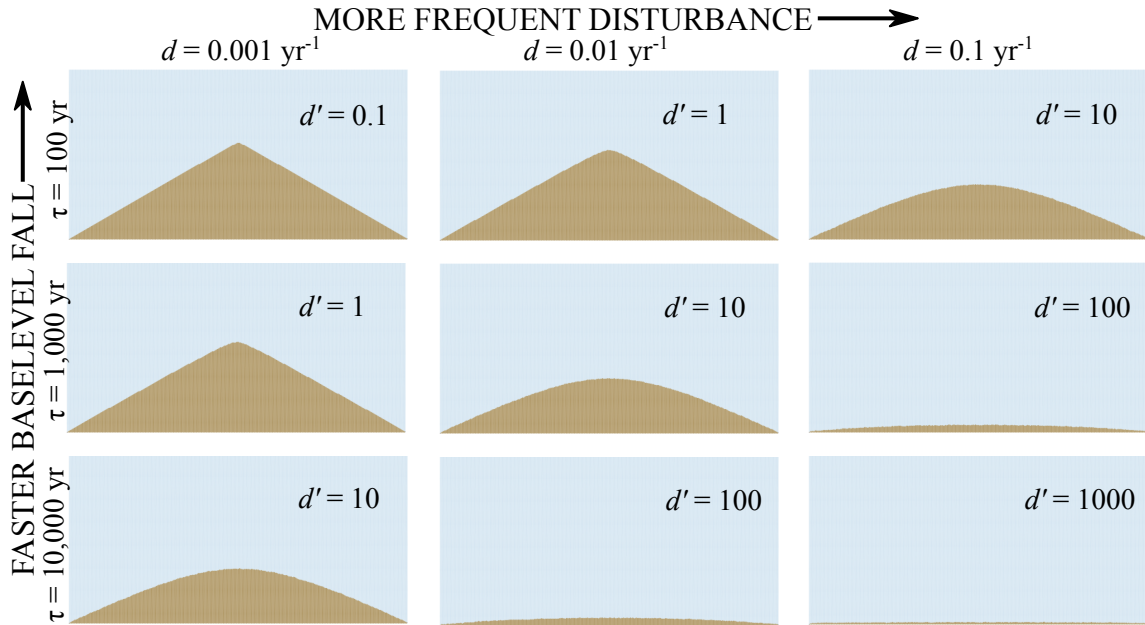
Figure 8. Equilibrium topographic cross-sections using only regolith particles (no rock) and a variety of disturbance frequencies ( d ) and time interval between baselevel fall events ( \tau ). Fast basal incision and/or infrequent disturbance leads to planar threshold hillslopes; slow basal incision and/or frequent disturbance leads to parabolic hillslopes.
