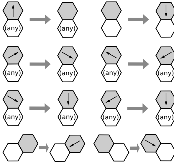
Figure 5. Illustration of gravitational rules. The bottom row shows the “falling on a slope” rule, which effectively imposes a 30^\circ angle of repose. Modified from Tucker et al. (2016).
