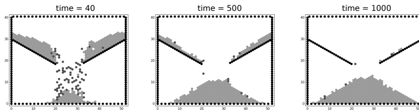
Figure 6. Lattice Grain simulation of emptying of a silo. Light-shaded grains are stationary; darker-shaded ones are in motion. Black cells are walls (rock). From Tucker et al. (2016).
