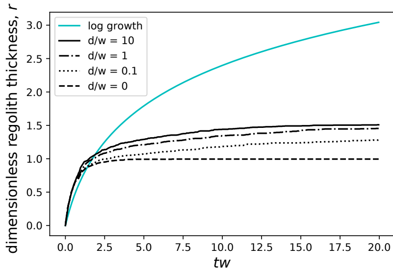
Figure 14. Regolith thickness versus time, as predicted by inverse-exponential theory (log growth; solid cyan curve) and the Grain Hill model with a range of ratios of disturbance rate ( d ) to weathering rate ( w ). Time (horizontal axis) is nondimensionalized by multiplying by w .
