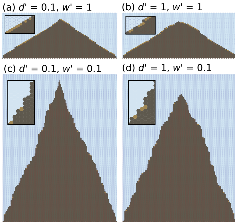
Figure 16. Quasi-steady model hillslope profiles created using a collapse rule, under four different combinations of d' and w' . Insets show magnified views of a portion of each hillslope.
