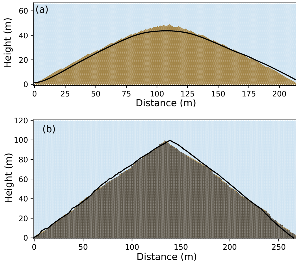
Figure 19. Steady state models using parameters estimated from observed hillslope profiles. (a) Parameters based on Gabilan Mesa, with the profile shown in Figure 2a,b for comparison. (b) Parameters based on Yucaipa Ridge, with the profile shown in Figure 2c,d for comparison.
