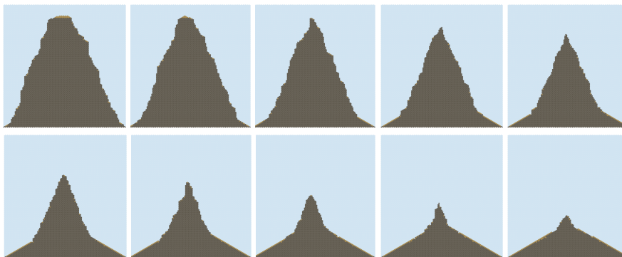
Figure 17. Time series showing transient erosion of a steep rock slope under a stable baselevel, highlighting formation of ramp-and-cliff morphology. Simulation shows 20,000 years of slope evolution under d = w = 10^{-3} \text{ y}^{-1} . Nominal width, assuming \delta = 0.1 \text{ m} , is 12 m.
