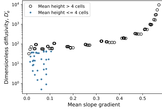
Figure 10. Relationship between dimensionless diffusivity and mean gradient, from the series of 125 model runs of which a subset are shown in Figure 8.
