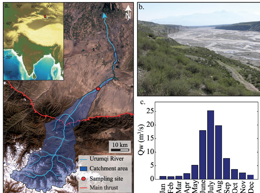
Figure 2. a) Location, drainage network and catchment area of the Urumqi River system, b) picture of the river at the sampling site during the high flow season ( the channel is ~300-m wide ), and c) annual hydrograph of the river (after Zhou et al., 1999).
