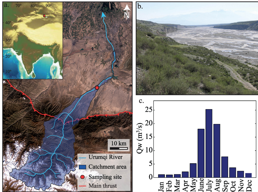
Figure 2. a) Location, drainage network and catchment area of the Urumqi River system, b) picture of the river at the sampling site during the high flow season (the channel is ~300-m wide), and c) annual hydrograph of the river (after Zhou et al., 1999).
