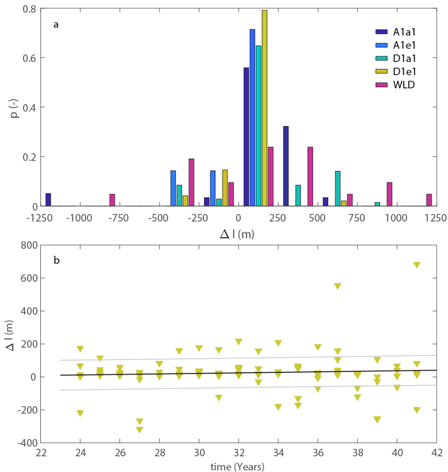
Figure 6. (a) Histogram of \Delta l for numerical model A1a1 (dark blue), A1e1 (light blue), D1a1 (seafoam) and D1e1 (yellow) compared with measurements from the Wax Lake Delta (pink). All histograms are binned at 250 m intervals. Descriptive statistics of these populations are shown in Table 2. (b) The location of \Delta l as a function of time (model years) for delta run 'D1e1.' A linear fit (black line) with 50% confidence interval (gray lines) are shown. The trend of this fit is not statistically significant, and small compared to variation within \Delta l .
