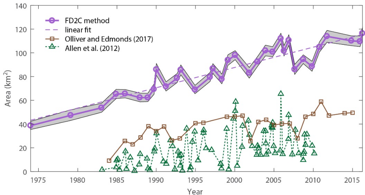
Figure 9. Area of the Wax Lake Delta as a function of time. Purple circles show the growth of the subaqueous Wax Lake Delta using the FD2C method. The gray region shows the 1\sigma deviation (16th to 84th percentile) of area found from Monte-Carlo sampling of \Delta I (Section 4.1). The dashed line shows the linear fit, with a growth rate of 1.72 \pm 0.13 \text{ km}^2/\text{yr} . Brown squares and green triangles show the subaerial growth as documented by Olliver and Edmonds (2017) and Allen et al. (2012).
