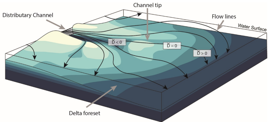
5 Figure 2: Schematic diagram of delta front morphology and streakline behavior. The colormap shows topography with dark colors representing deep areas and light colors representing shallow or subaerial areas. Streaklines are shown as black solid lines. The FD2C method takes advantage of flow direction divergence ( \bar{D} < 0 ) through the shoaling reach of the channel and lateral flow direction convergence ( \bar{D} > 0 ) on the basinward sloping delta front. The channel tip occurs roughly when \bar{D} transitions from negative to positive.
