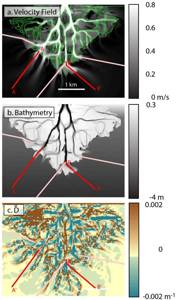
5 Figure 4. Method for comparing \check{D} to bathymetry using a Delft3D numerical simulation (run A1e1). (a) The velocity field and -0.3 m MSL (green) contour are displayed and transects (pink and red lines) are drawn extending from the largest distributary network channels. (b) The bathymetric profile is collected along each transect. (c) \check{D} is calculated, and transects of \check{D} are collected along the transects. Transects A-A' and B-B' are shown in Figure 5.
