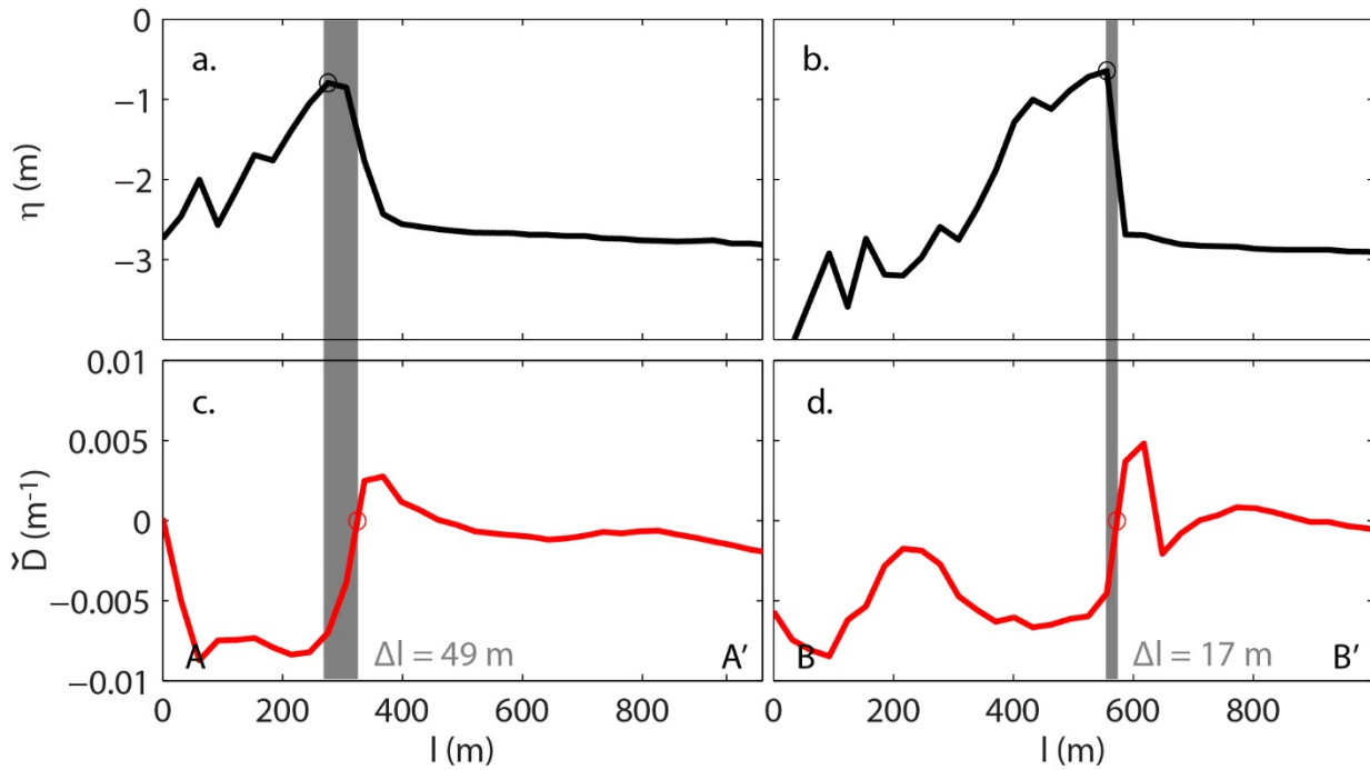
Figure 5. Comparison of bathymetry ( \eta ; plots a and b) and divergence of flow direction ( \bar{D} ; plots c and d) for transects A-A' (plots a, c) and B-B' (plots b, d). \Delta l is the width of the gray box, or the location where \bar{D} changes from positive to negative ( x_{\bar{D}} ; red circle) minus the bathymetric maximum of the channel tip ( x_{\eta} ; black circle). The distribution of \Delta l is shown in Figure 6.
