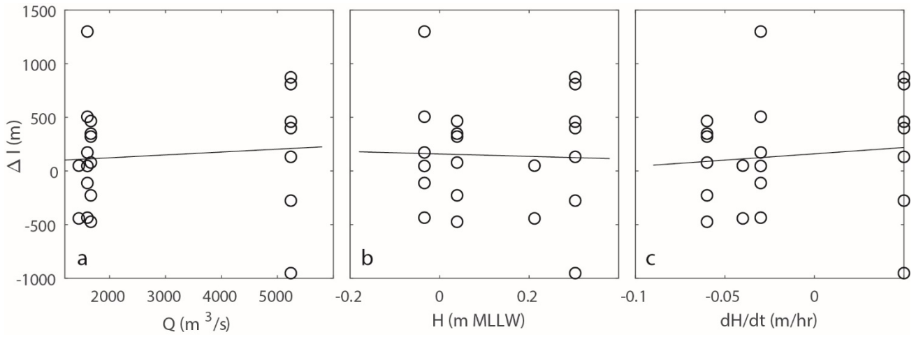
Figure 7. Comparison of \Delta l measurements on the WLD to unsteady hydrodynamic conditions. In each case, the black line shows the linear trend, which is negligible. (a) shows upstream water discharge, with r^2 = 0.01 . (b) shows tidal elevation relative to mean lower low water with r^2 = 0.001 , (c) shows rate of change of tide elevation averaged over 30 minutes with r^2 = .01 .
