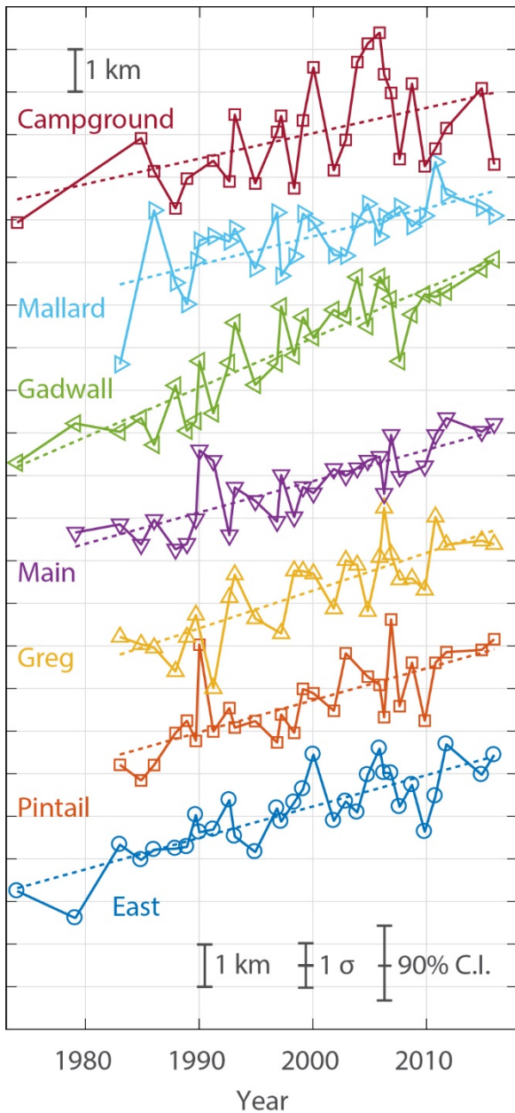
Figure 8. Growth of individual channels over time. Each series is plotted at the same scale (horizontal lines = 1 km, vertical lines 10 years), but are shifted vertically for clarity. The uncertainty associated with \Delta l measured at Wax Lake Delta (Figure 6a) is shown with a standard deviation ( \sigma ) and 90% confidence interval (C.I.) at the bottom. The primary distributary channels are shown from West to East: Campground Pass (maroon squares), Mallard Pass (turquoise right-pointing triangles), Gadwall Pass (green left-pointing triangles), Main Pass (purple down-pointing triangles), Greg Pass (yellow up-pointing triangles), Pintail Pass (red squares), and East Pass (blue circles). Dashed lines show linear regressions of each dataset.
