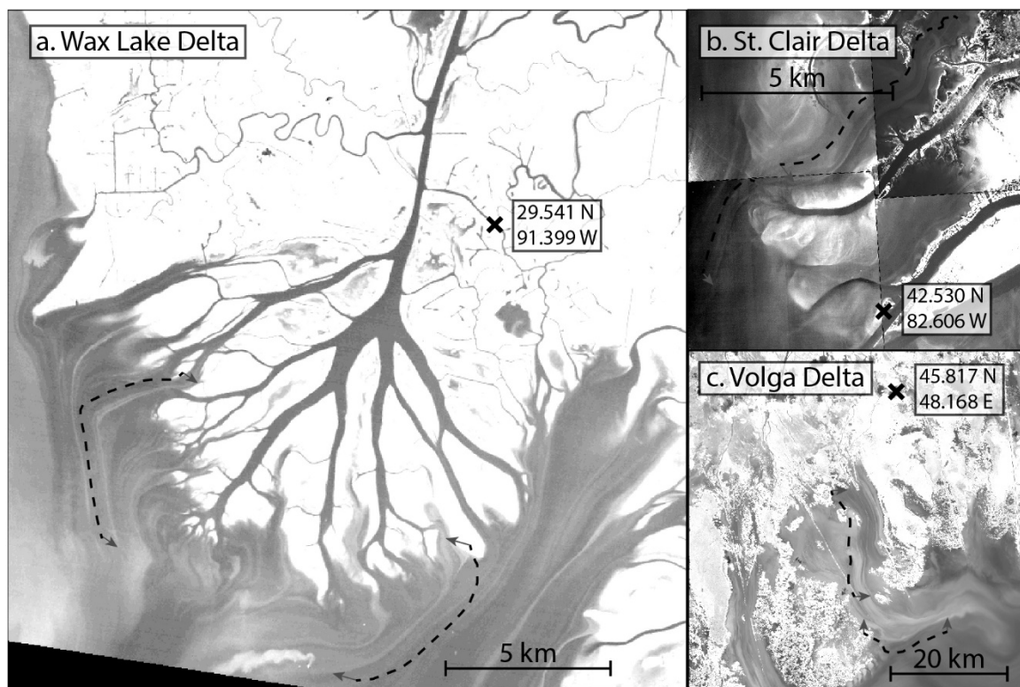
Figure 1: Images of river deltas exhibiting streaklines. (a) Wax Lake Delta (Landsat image LT50230402011002CHM01 Band 4). (b) the Saint Clair Delta in Michigan, USA (Digital Orthophoto Quads Saint Clair Flats NE, NW, SW, SE, IR band). (c) Portion of the Volga Delta in Russia (Landsat LC08_L1TP_168028_20170501_01 Band 4). In each image, streaklines are mapped in dashed lines. The line is translated in space slightly (see gray arrows) to reveal the streakline in the image.
